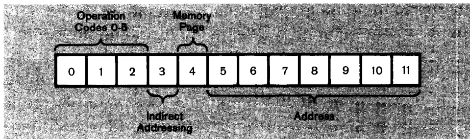
Figure 5 Memory Reference Instruction Bit Assignments
