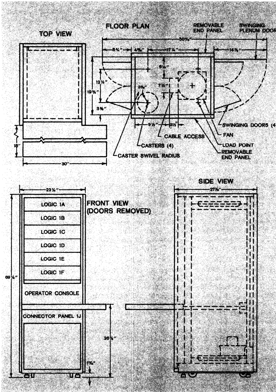
Figure 11 Component Location and Installation Diagram
