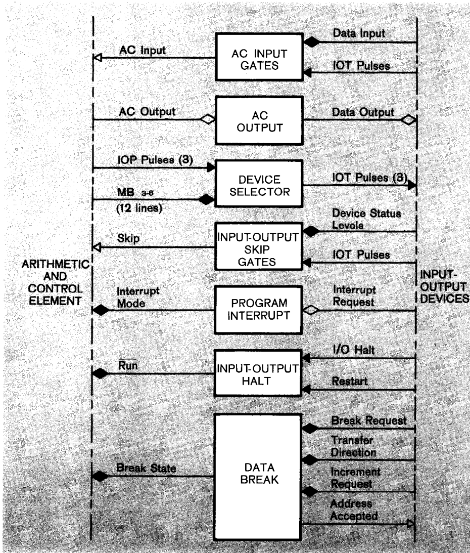
Figure 9 Input-Output Control Element
