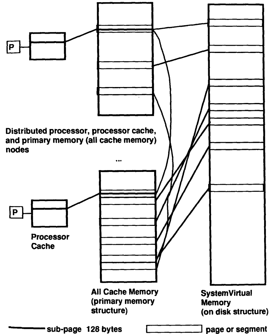
Fig. 5. Structure of a distributed shared memory "all cache" architecture.
