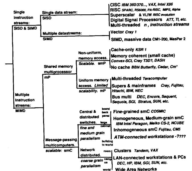
Fig. 2. Computer taxonomy showing parallel and scalable structures.
