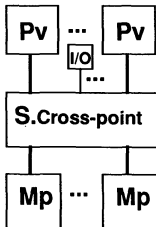
Fig. 3. Multiple vector processor supercomputers (e.g. Cray, IBM, Fujitsu, Hitachi, NEC).
