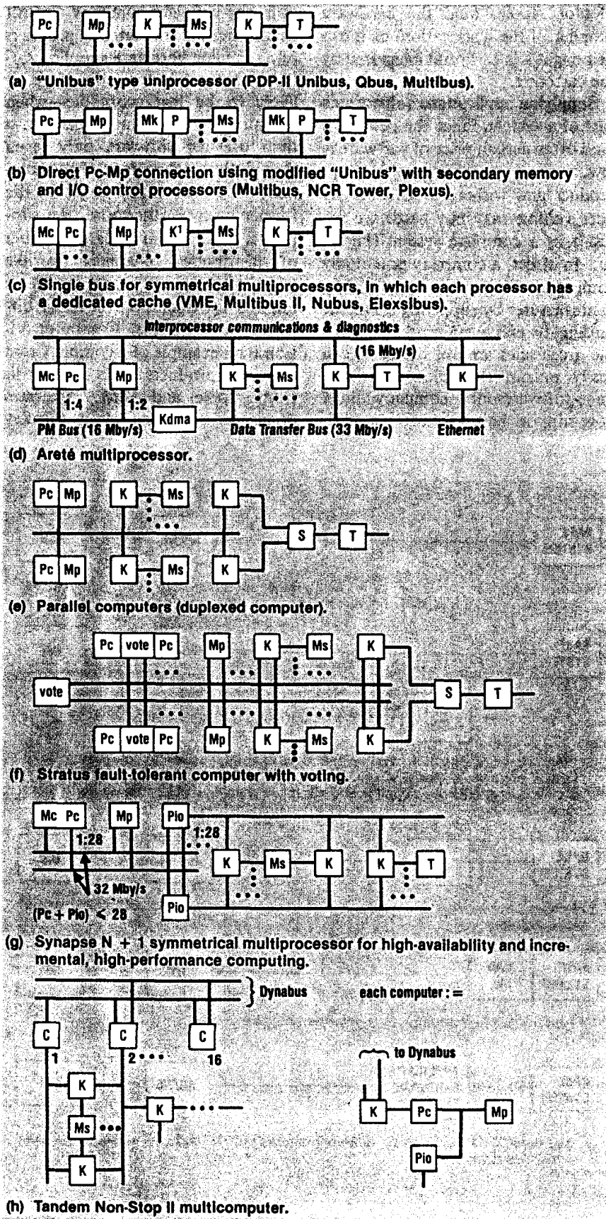
Figure A-1. Common micro- and mini-computer structures. Pc = central processor; Pio = i/o processor; K = control; Mp = primary memory; Mc = cache; Ms = secondary memory; and T = transduce (terminal).
