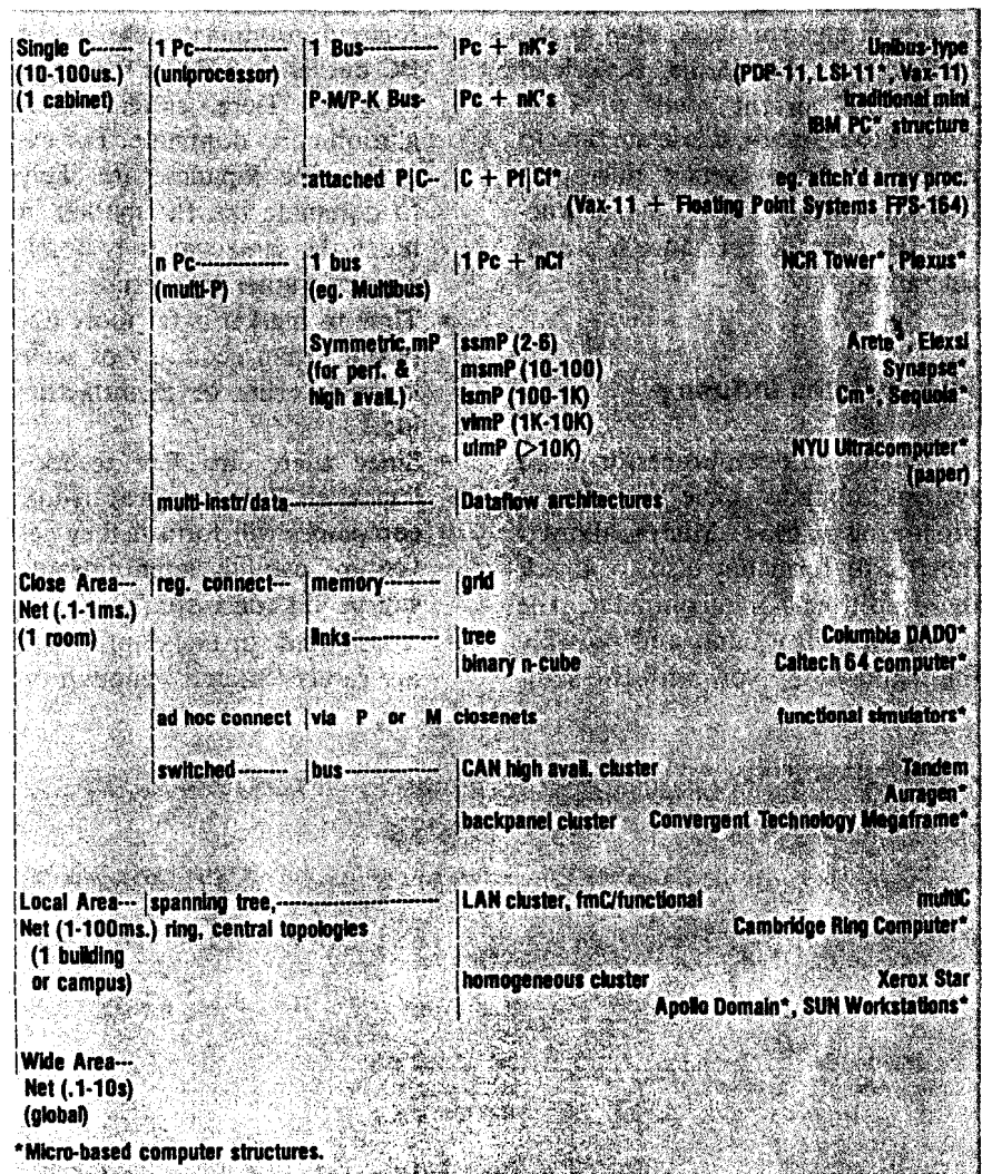
Figure 3. Taxonomy of common mini- and micro-based computer structures. C = computer; P = processor; K = controller; Cluster = collection of C's acting as a single C—interprocessor communication times determine parallel processing grain size; and function = arithmetic, array processor, signal processor, communication (front end), database (back end), display, simulation.
