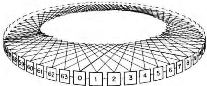
This routing diagram shows schematically the neighbor-to-neighbor linkages which form the 64 processing elements (PE) into a ring, as well as the connections of the PE's eight apart such that data can bypass intermediate PE's when the distance to be covered is large.
