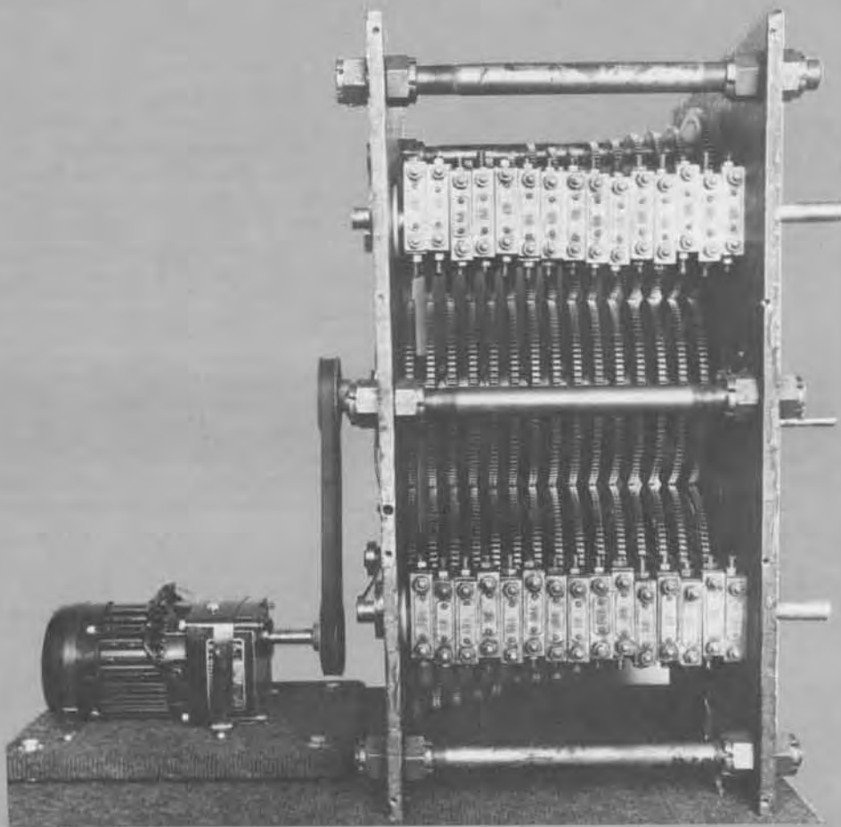
This Photoelectric Number Sieve, built by Dr. Lehmer in 1932, performs 300,000 tests per minute using 30 gears arranged tangentially. Each gear has a number of holes equal to a multiple of a prime. For any problem, all holes that do not represent solutions are plugged with toothpicks. A solution is found when light, originally supplied by an automobile headlight lamp, passes through all 30 wheels. A photoelectric cell detects this brief flash of light, and a vacuum-tube amplifier multiplies the resulting signal 700,000,000 times to stop the motor.
