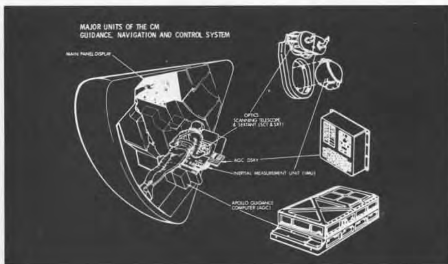
Major units of the CM Guidance, Navigation and Control System from the MIT Draper Lab.
