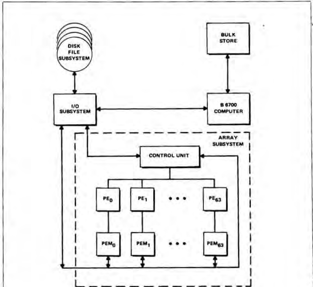
Illiac IV functional diagram.
