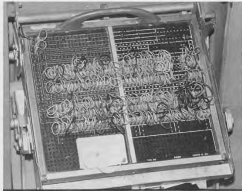
Plugboard Program Central Unit.
