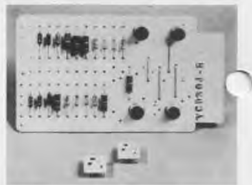
Two COMPAC Modules (bottom), Equivalent to the Standard Modular System Card (top); 1961.
