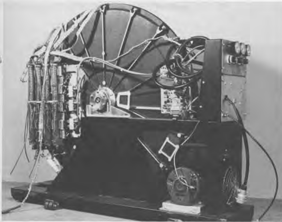
This Burroughs Disk exhibited at The Computer Museum is only one of the thirteen synchronously rotating fixed head disks that comprised the 16M word main memory of Iliac IV.
