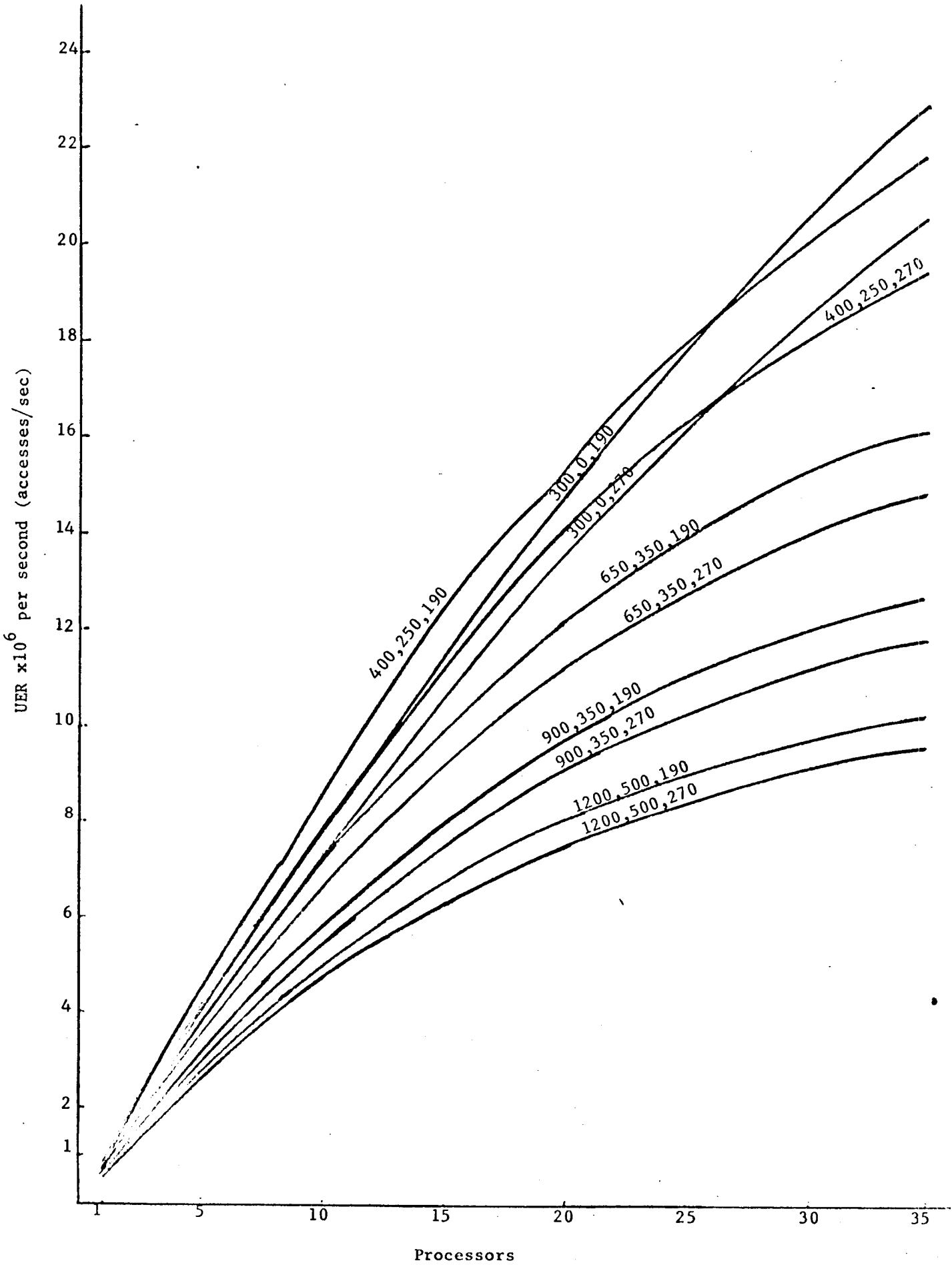
Fig. 4d. Performance vs Pc's for 16 Mp; Pc(Model 20; tp 700 ns)
