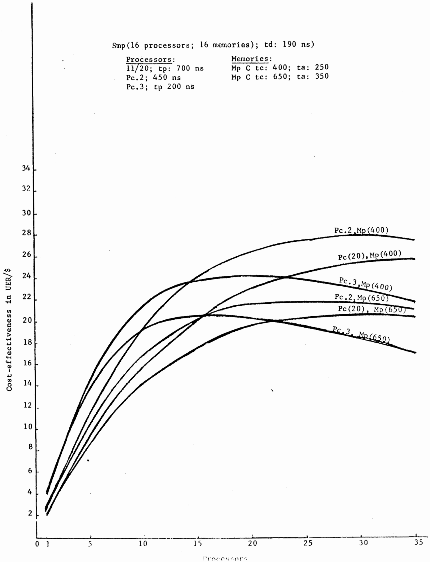
Fig. 5. Cost effectiveness (UER/$) vs Pc's.
