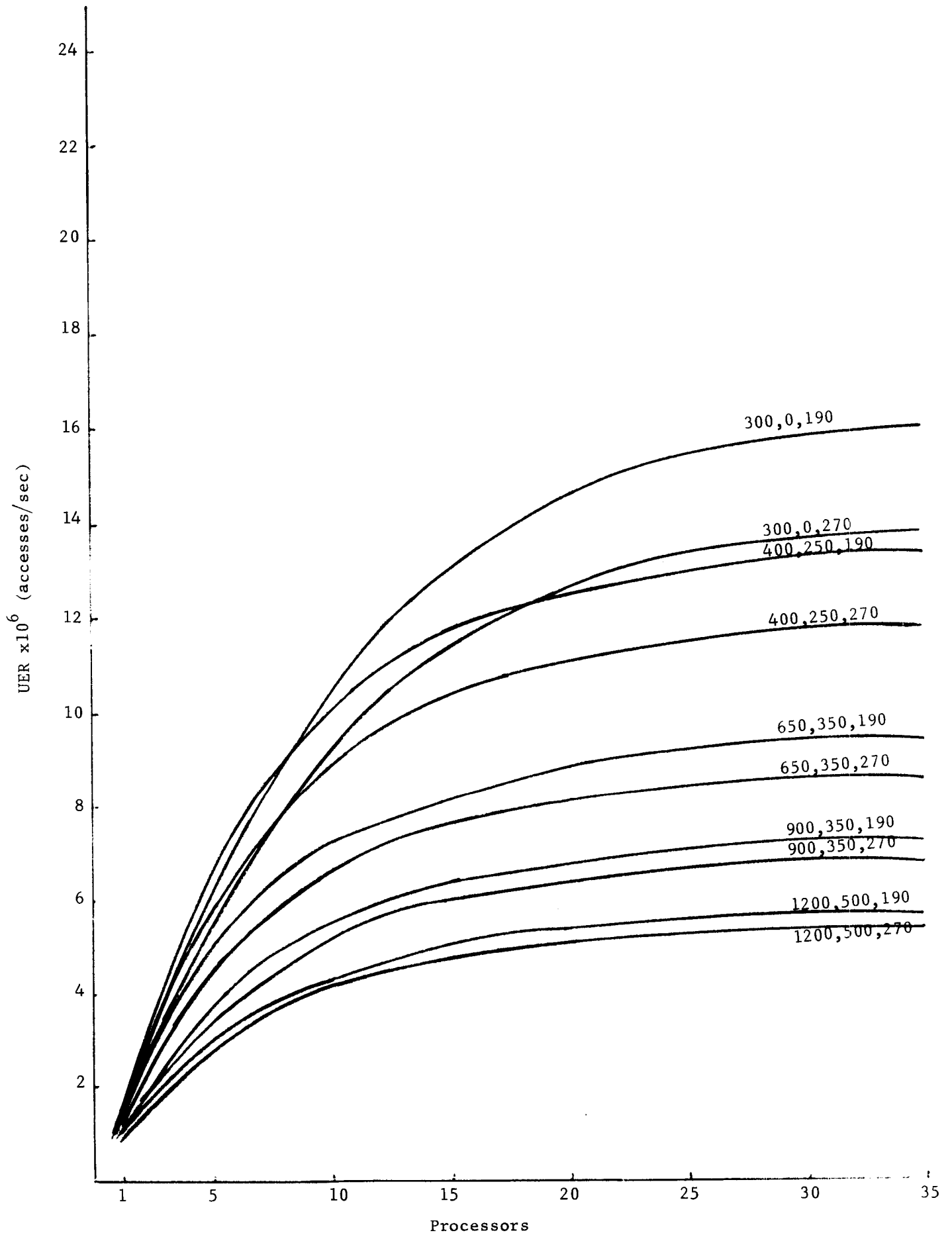
Fig. 4c. Performance vs Pc's for 8 Mp; Pc(#3; tp: 200 ns)
