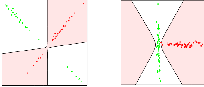
FIG. 3.1. MICL harnesses the covariance structure of the data to interpolate (left) and extrapolate (right) in regions where the training samples are sparse.
