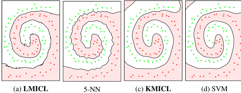
FIG. 5.2. Comparison of nonlinear extensions to MICL against SVM and k -NN. Notice that local MICL improves upon k -NN, producing a smoother and more intuitive decision boundary. Kernel MICL and SVM produce similar boundaries, that are smoother and better respect the data structure than those given by either of the local methods.
