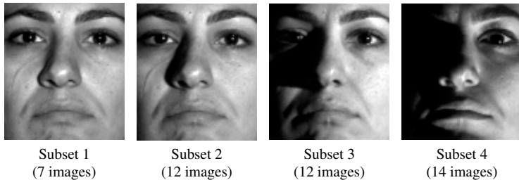
FIG. 5.4. The Extended Yale B Face Database includes 1,694 images of 38 subjects under varying illumination. The database is divided into four subsets taken under increasingly extreme lighting conditions. In our experiments, we train using Subset 1, and test with each of the remaining subsets.
