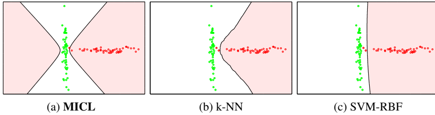
FIG. 5.1. Extrapolation of data structure. Left: MICL. Center: 5-NN. Right SVM-RBF.
