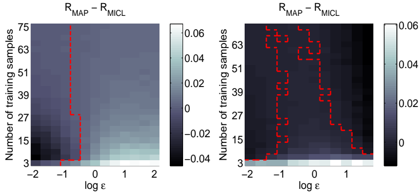
FIG. 3.2. Excess misclassification risk incurred by using MAP rather than MICL, as a function of \varepsilon and m . MICL outperforms MAP in most settings, with the largest gain when m is relatively small. Left: two isotropic Gaussians in \mathbb{R}^2 . Right: anisotropic Gaussians in \mathbb{R}^2 .
