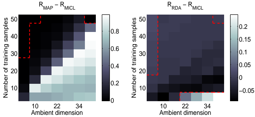
FIG. 3.3. Excess risk incurred by using MAP and RDA rather than MICL, as a function of number of samples m and dimension n .
