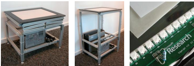
Figure 4: (i) Table in its collapsed state, (ii) ready for use, and (iii) close up of edge lit IR LED illumination, acrylic sheet, latex sheet and drafting film.
