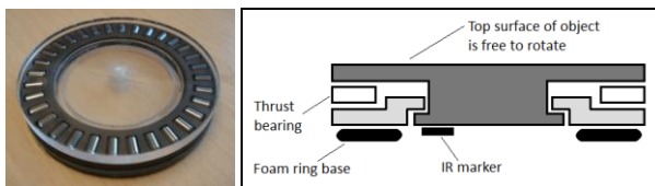
Figure 5: Tangible 'scratching' object.
