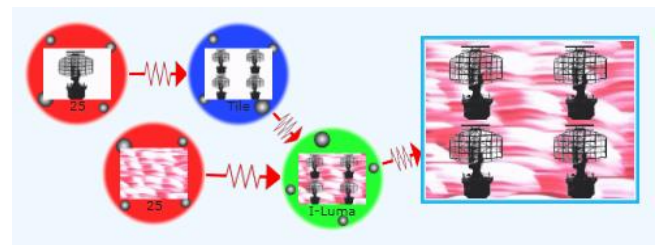
Figure 3: The VPlay user interface. In this example, two video clips (on the left) are connected to a display object (on the right) via an inverse luma key mixer and a 'tile' effect object.
