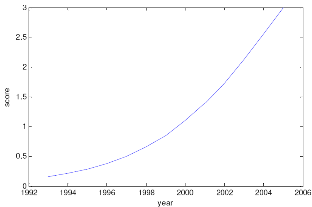
Figure 1: Scoring function for the query-independent feature Year.
