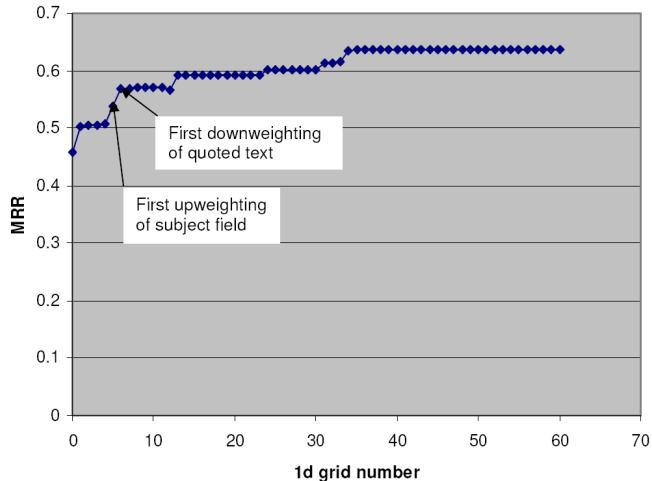
Figure 2: Ten rounds of tuning the six BM25F parameters gave these 60 MRR values on the training set (and the left-most untuned point). The tuning order was: B_{Body} , B_{Subject} , B_{Quoted} , W_{Body} , W_{Subject} , W_{Quoted}
