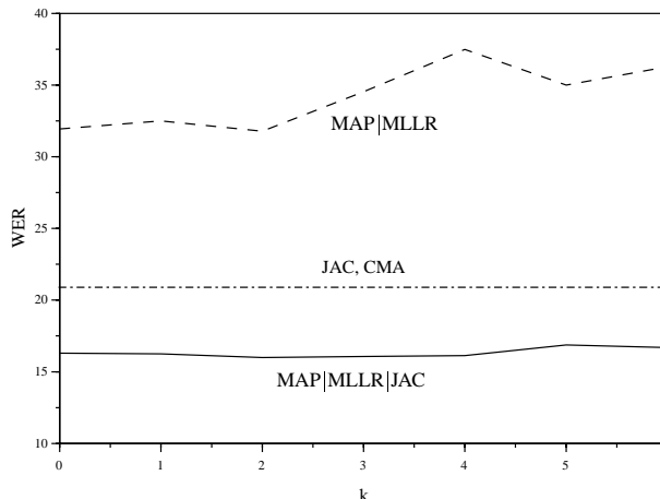
Figure 1: Word error rates for speaker adaptation and for joint speaker adaptation and noise compensation with different interleaving lengths.
