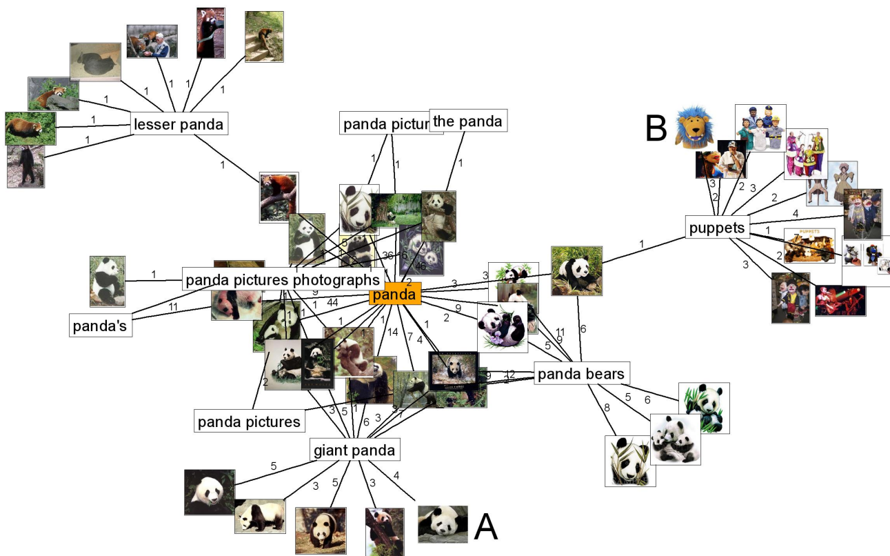
Figure 1: Click graph. Nodes are queries or images, edges indicate clicks. Images A and B are equidistant from the query ‘panda’ (distance=3), so retrieval based on a naïve shortest-path algorithm could not distinguish them. Our Markov random walk approach sums over paths, so image A benefits from having 7 distinct paths of length 3. In other words, nodes A and ‘panda’ are connected by a large “volume” of paths.
