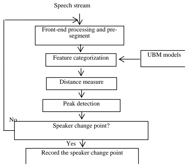
Figure 1. A brief flow diagram for speaker change detection
