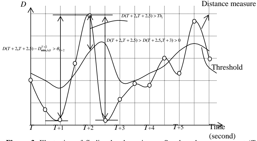
Figure 3. Illustration of finding local maximum. Speaker changes occur at (T+2) and (T+5.5).
