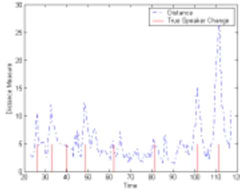
Figure 9. Real time Speaker segmentation based on distance measure
