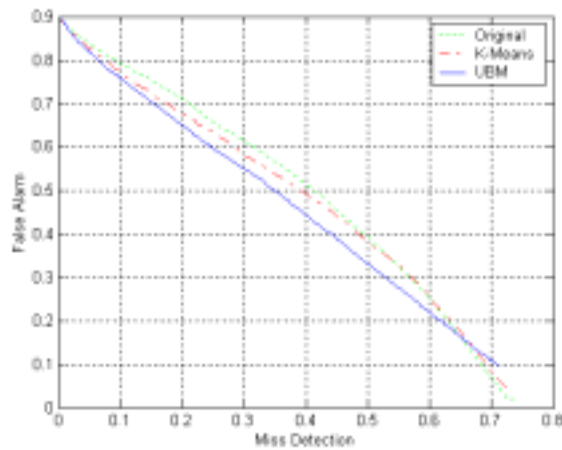
Figure 6. The ROC curves of three approaches with MFCC feature
