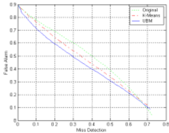
Figure 5. The ROC curves of three approaches with LSP feature
