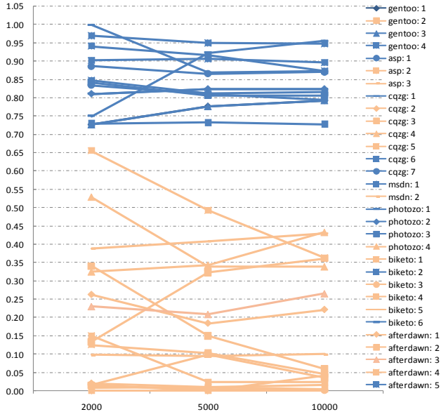
Fig. 10. The connectivity scores of all the loop-back links with different numbers of sampled pages. Page-flipping links are marked in blue and non page-flipping links are in orange.
