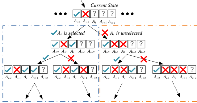
Fig. 4. An illustration of the search process of skeleton links.
