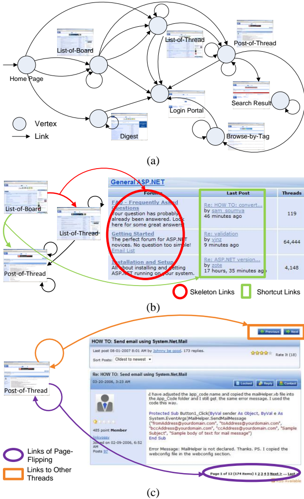
Fig. 1. An illustration of the (a) Sitemap, (b) Skeleton Link, and (c) Page-Flipping Link. The graph in (a) and the screen shots in (b) and (c) have been simplified for a clear view.
