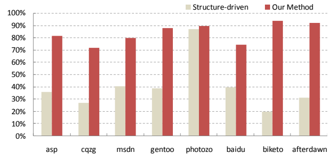
Fig. 7. The coverage of valuable pages retrieved by the structure-driven crawler and our method.
