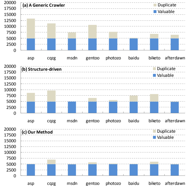
Fig. 9. The comparison of efficiency between (a) the generic crawler, (b) the structure-driven and (c) our method, to retrieve 5,000 valuable pages.
