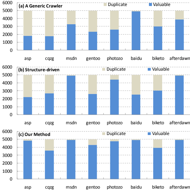
Fig. 8. The comparison of effectiveness between (a) the generic crawler, (b) the structure-driven crawler and (c) our method, on the top 5,000 retrieved pages.
