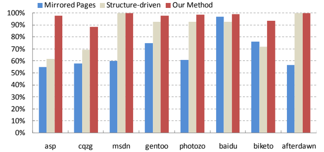
Fig. 6. The comparison of informativeness for the mirrored pages and, the pages crawled by our method and the structure-driven crawler, on various forums, respectively.
