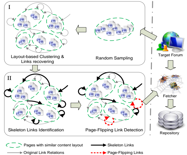
Fig. 2. The flowchart to the proposed approach, which consists of two parts: (I) sitemap recovering; and (II) traversal strategy exploring
