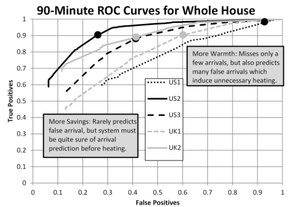
Figure 8: These ROC curves demonstrate the tradeoff in prediction mistakes that come from adjusting the probability threshold.
