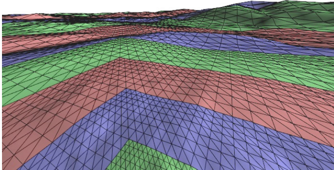
Illustration using a coarse geometry clipmap (size n=31 )
