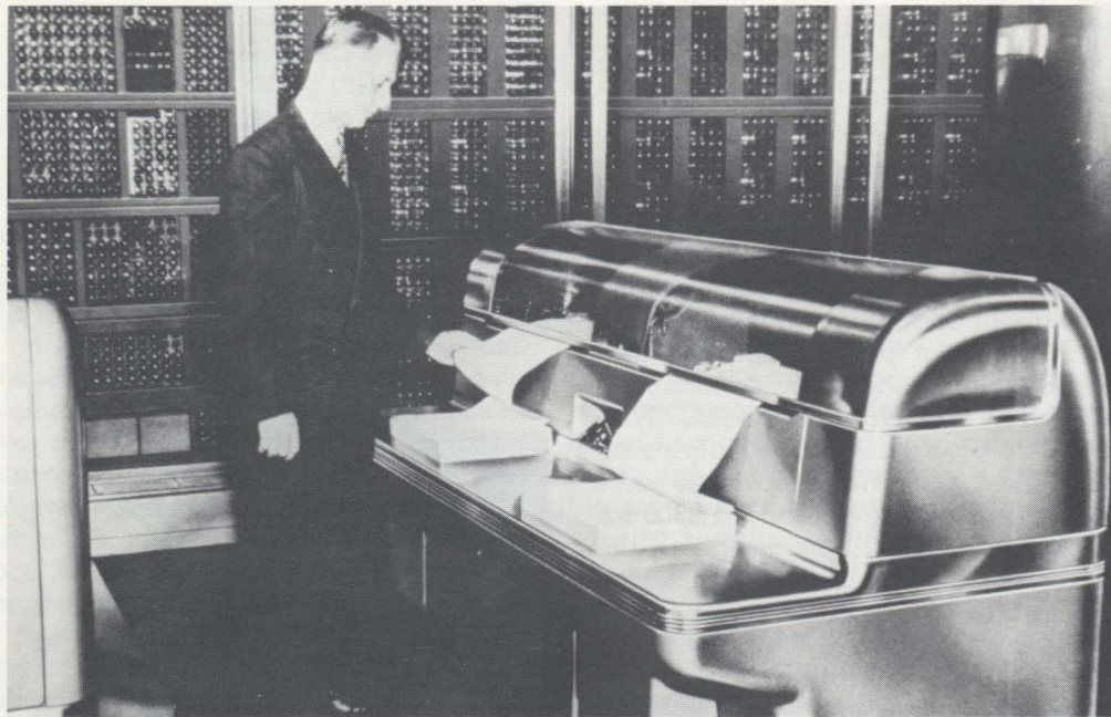
The SSEC used conventional IBM 405 tabulators rehoused with the tape slugs turned upside down and the wires crossed so as to make it work out of the back instead of the front for the sake of appearance. The 12,000 inch and a quarter diameter 25L6 boggles out of which the arithmetic circuits were made can be seen in the back of the photo.
