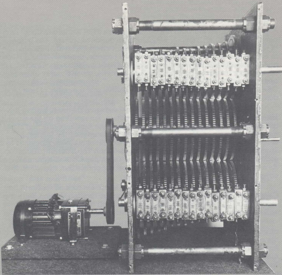
This Photoelectric Number Sieve, built by Dr. Lehmer in 1932, performs 300,000 tests per minute using 30 gears arranged tangentially. Each gear has a number of holes equal to a multiple of a prime. For any problem, all holes that do not represent solutions are plugged with toothpicks. A solution is found when light, originally supplied by an automobile headlight lamp, passes through all 30 wheels. A photoelectric cell detects this brief flash of light, and a vacuum-tube amplifier multiplies the resulting signal 700,000,000 times to stop the motor.
