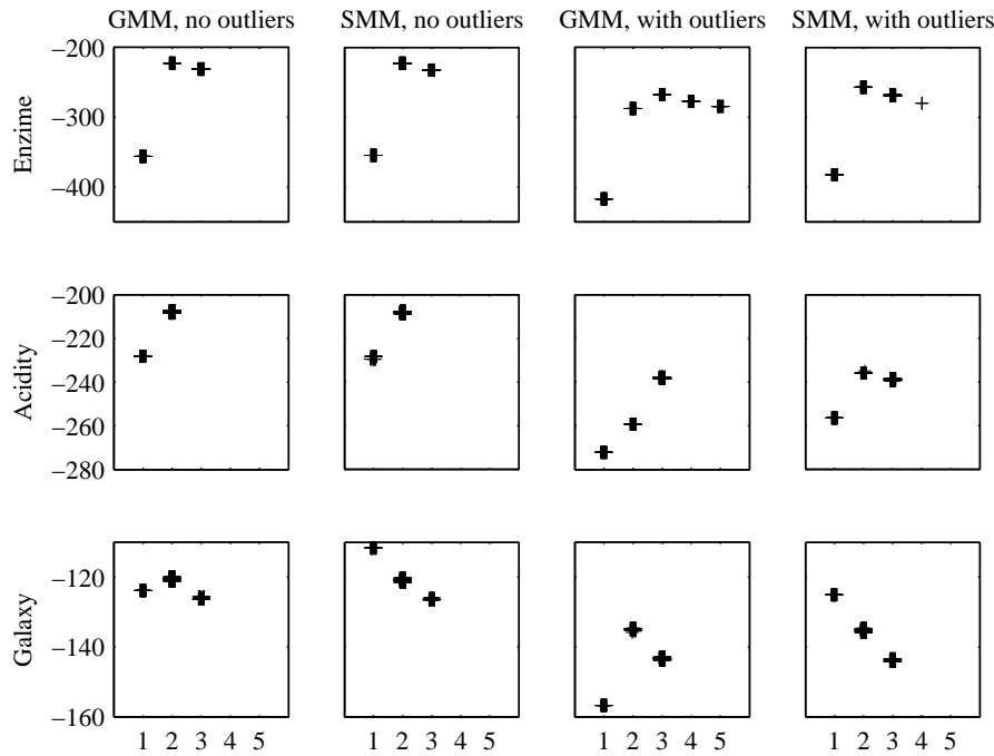
Figure 2: Comparison of Gaussian (GMM) and Student (SMM) mixture models in their robustness to outliers on three different data sets, showing plots of the lower bound of the fitted model versus the effective number of components. All plots share the same horizontal range of [0, 6] and all plots on the same row have the same scale on the vertical axis. Each solution is plotted as a '+'-sign and a small amount of uniform noise has been added to its horizontal position, in order to make the results visually clearer.
