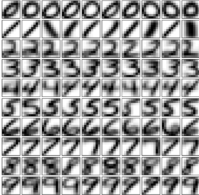
Figure 9: The mean vectors \mu_i , illustrated as gray-scale digits, for each of the ten digit models. The model for a given digit is a mixture of ten PCCA models, one centred at each of the pixel vectors shown on the corresponding row. Note how different components can capture different styles of digit.
