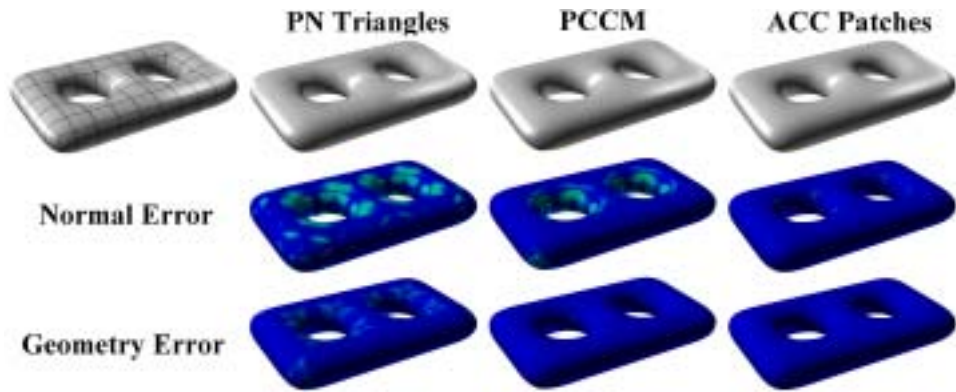
Fig. 18. Comparison of our method with PN-Triangles and PCCM on a two-hole torus containing only odd valence extraordinary vertices after one level of subdivision. Our ACC-Patches provide superior approximation both in terms of the normals of the surface as well as its geometry.
