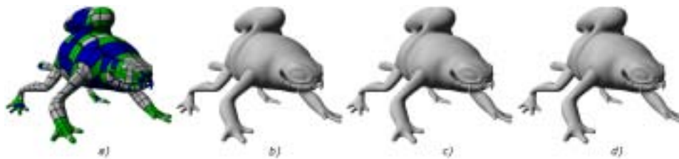
Fig. 8. a) The patch structure we associate with a Catmull-Clark subdivision surface. The grey patches contain only valence 4 vertices, green have one extraordinary vertex and blue have more than one extraordinary vertex. b) Our approximation to the Catmull-Clark subdivision surface using geometry patches and c) our final approximation using geometry and tangent patches compared with d) the actual Catmull-Clark limit surface.
