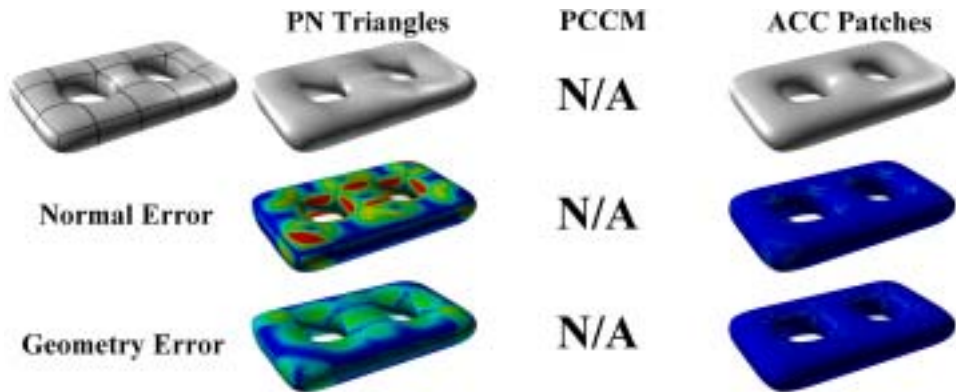
Fig. 17. Comparison of our method with PN-Triangles and PCCM on a two-hole torus containing only odd valence extraordinary vertices. There is not sufficient separation of extraordinary vertices for PCCM in this example.
