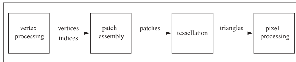
Fig. 19. Proposed future GPU pipeline.
