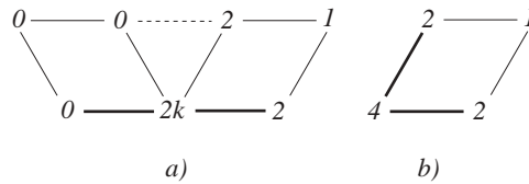
Fig. 21. Rules for creating the interior Bézier control point adjacent to a boundary vertex contained by more than one quad a) and only one quad b) .
