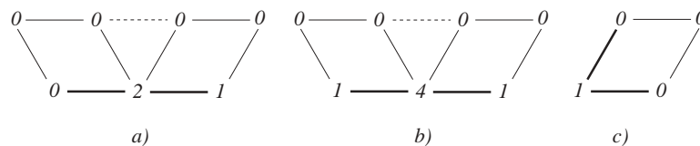
Fig. 20. Rules for Bézier control points along the boundary to create a cubic B-spline. Bolded edges indicate boundaries. From left to right: mask for an edge control point, corner control point and a corner control point contained by only one quad.
