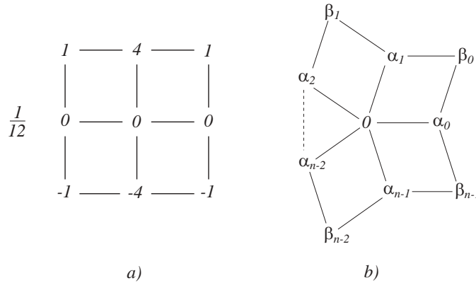
Fig. 6. a) Tangent mask for uniform bicubic B-splines surfaces b) Mask for Catmull-Clark limit tangent.
