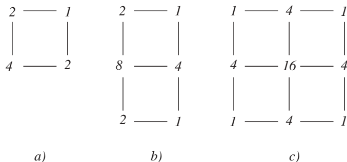
Fig. 3. Masks for determining Bézier control points from a uniform bicubic B-spline surface.
