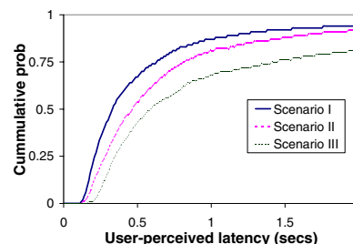
Figure 16: CDF of User-perceived page latency
