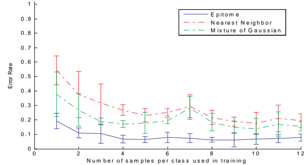
Figure 8: Error vs. number of training examples.
