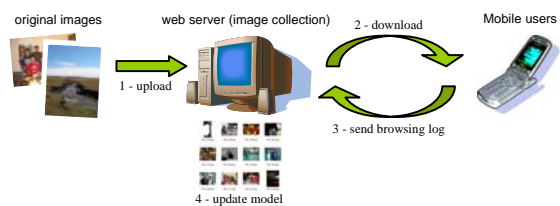
Figure 10. Collaborative update of the image attention model.
