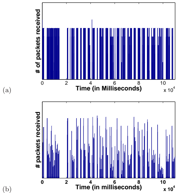
Figure 5: Pictorial proof of ON/OFF characteristics: Time series of Data Center traffic (number of packets per time) binned by three different time scales. Traffic in figure (a) is binned by 15ms and by 100ms in (b).
