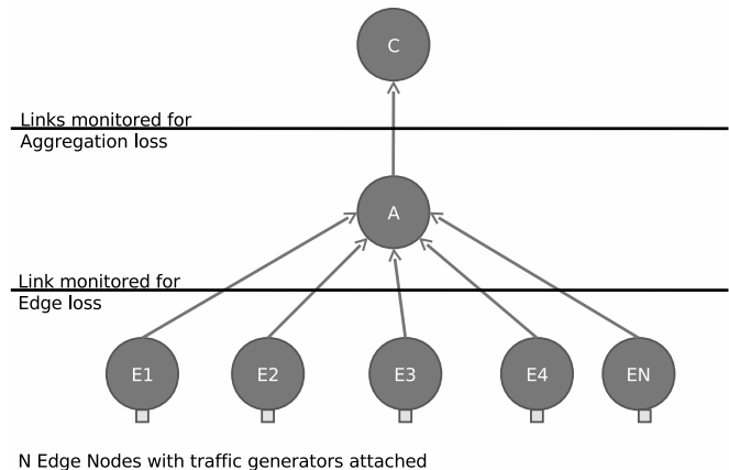
Figure 10: Topology simulated in deriving loss patterns.
