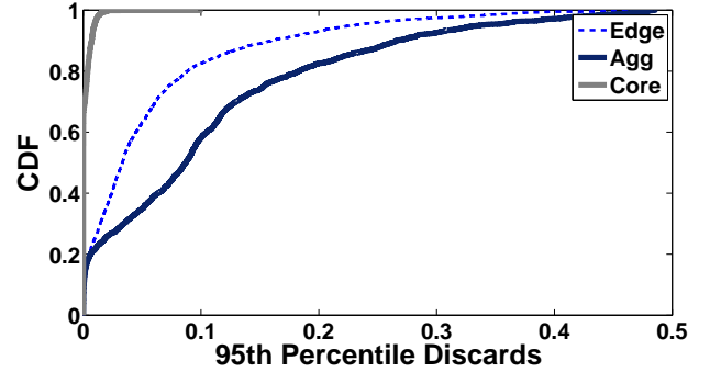
Figure 3: CDF of 95th percentile “scaled” loss rates of links at the various layers in all data center.
