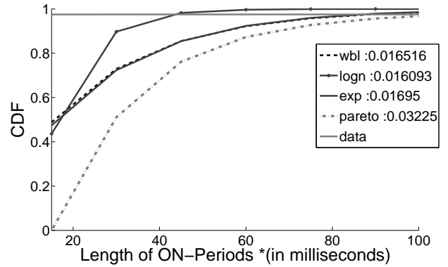
Figure 8: CDF of the distribution of the ON-Period lengths at one of the switches in DC 10. The figure contains best fit curve for lognormal, weibul, pareto, and exponential as well as the least mean errors for each curve. We notice that the lognormal fit produces the least error
