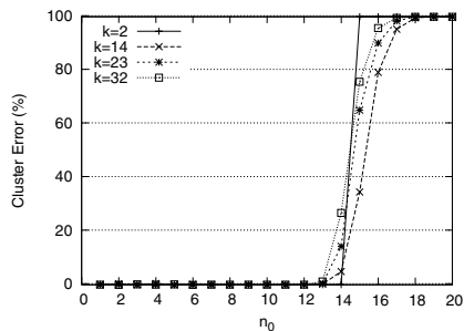
Fig. 3: Percentage of overall cluster errors for different n_0, k, n_b = 32 .
