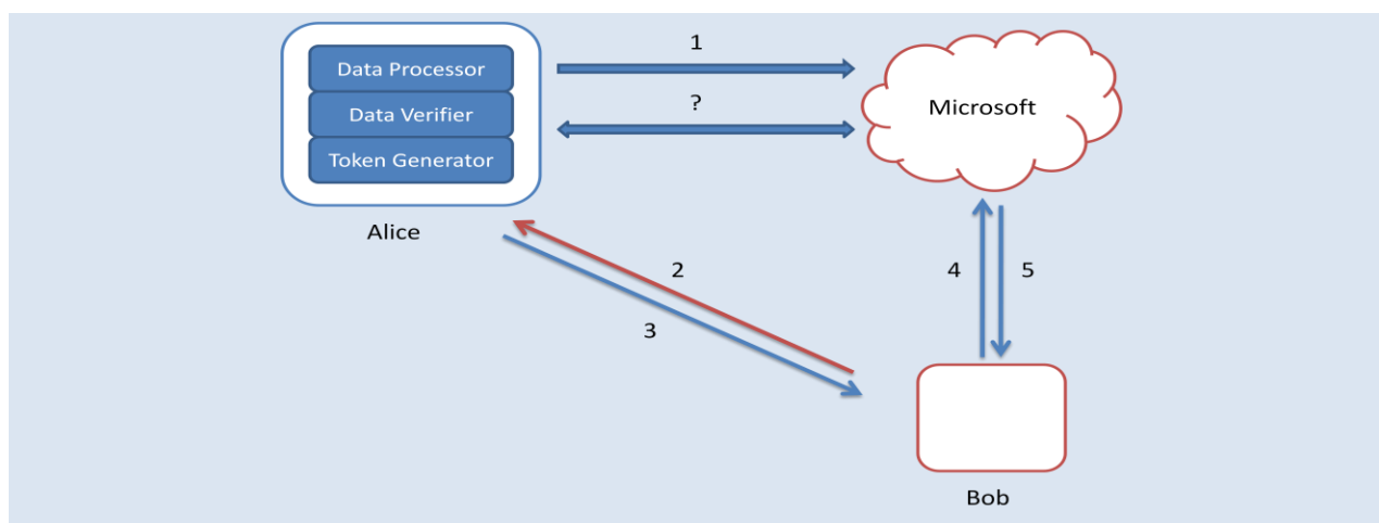
Figure 1: (1) Alice’s data processor prepares the data before sending it to the cloud; (2) Bob asks Alice for permission to search for a keyword; (3) Alice’s token generator sends a token for the keyword and a decryption key back to Bob; (4) Bob sends the token to the cloud; (5) the cloud uses the token to find the appropriate encrypted documents and returns them to Bob. At any point in time, Alice’s data verifier can verify the integrity of the data.
