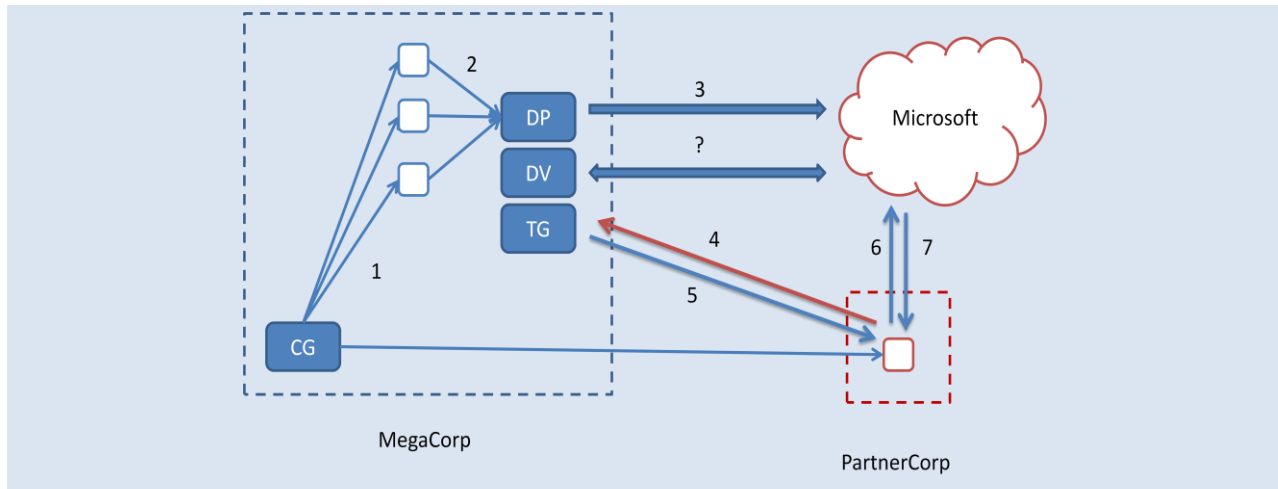
Figure 2: (1) Each MegaCorp and PartnerCorp employee receives a credential; (2) MegaCorp employees send their data to the dedicated machine; (3) the latter processes the data using the data processor before sending it to the cloud; (4) the PartnerCorp employee sends a keyword to MegaCorp's dedicated machine ; (5) the dedicated machine returns a token; (6) the PartnerCorp employee sends the token to the cloud; (7) the cloud uses the token to find the appropriate encrypted documents and returns them to the employee. At any point in time, MegaCorp's data verifier can verify the integrity of MegaCorp's data.
