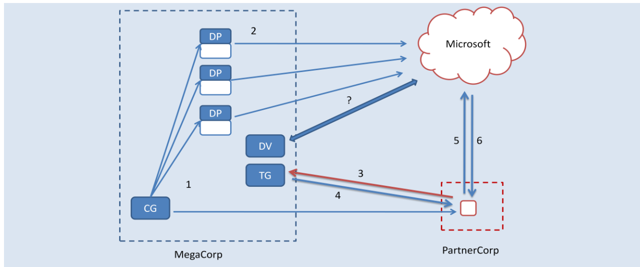
Figure 3: (1) Each MegaCorp and PartnerCorp employee receives a credential; (2) MegaCorp employees process their data using their own data processors and send them to the cloud; (3) the PartnerCorp employee sends a keyword to MegaCorp’s dedicated machine; (4) the latter returns a token; (5) the employee sends the token to the cloud; (6) the cloud uses the token to find the appropriate encrypted documents and returns them to the employee. At any point in time, MegaCorp’s data verifier can the integrity of MegaCorp’s data.
