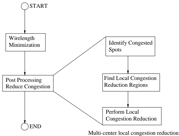
General congestion-driven placement
