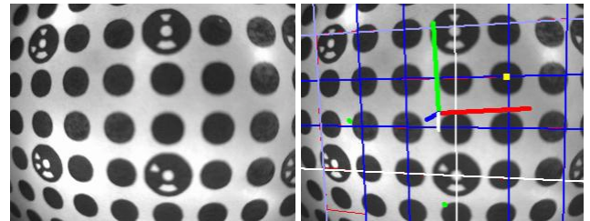
Fig. 4 The revised grid encodes position information in the large dots for better tracking of rapid 2D mouse motions.
