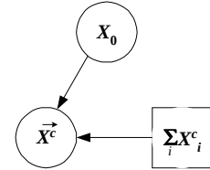
Figure 2: The multinomial model.
