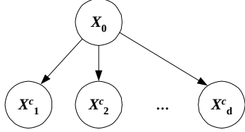
Figure 3: The Poisson naive Bayes model.
