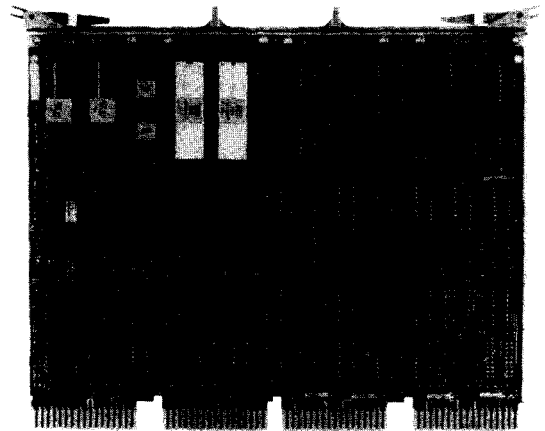
Figure 6. LSI-11 processor with 8 Kbytes of memory and microcode for commercial instruction set.
