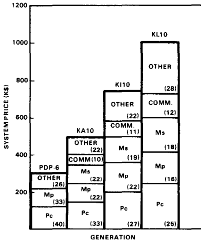
Figure 9. System component price versus generation.
