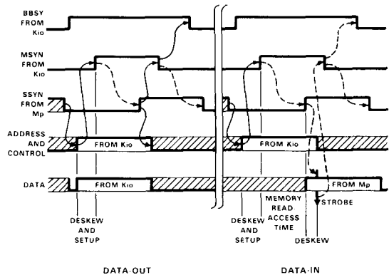
Figure 19. Timing diagram of transfers on Unibus.
