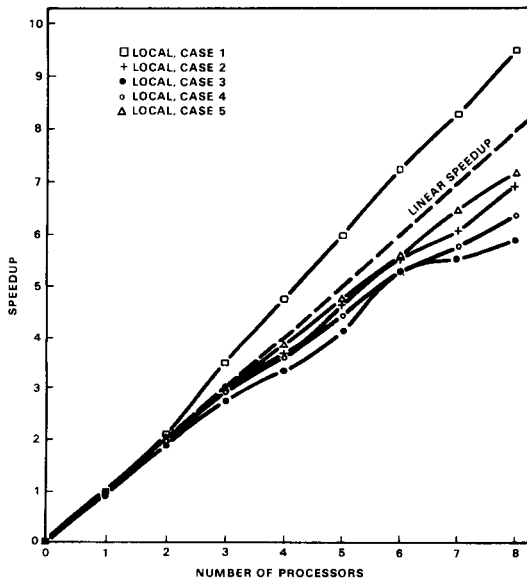
Figure 21. Integer programming speedup.
