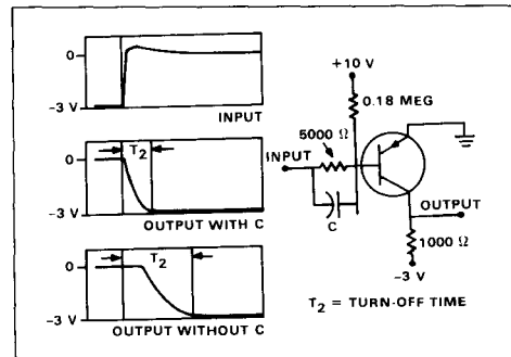
Figure 7. Turn-off time.
