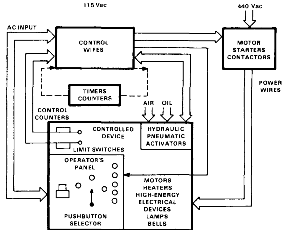
Figure 31. Hardwired machine for industrial control.
