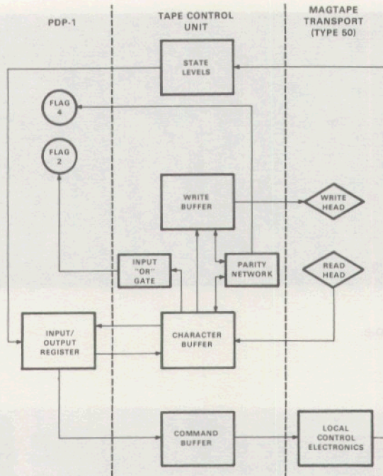
Figure 7. Program control-based magnetic tape control from PDP-1 register transfer diagram.
