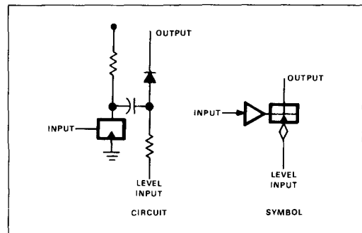
Figure 13. Positive C-D gate.
