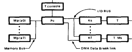
Figure 3. PDP-8 S(I/O Bus) logic and PMS diagrams.
