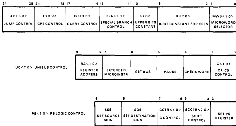
Figure 4. Microinstruction format.
