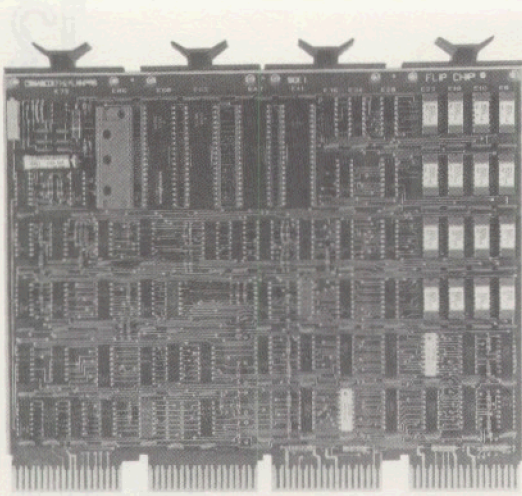
Figure 1. On one 21.6 cm X 26.7 cm board, the LSI-11 provides a complete PDP-11 processor, 4 Kwords of 16-bit memory, an ASCII console, a real-time clock, an automatic dynamic memory refresh, and interface bus control.
