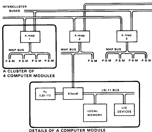
Figure 6. The basic structure of Cm*
