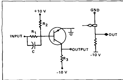
Figure 3. Inverter.
