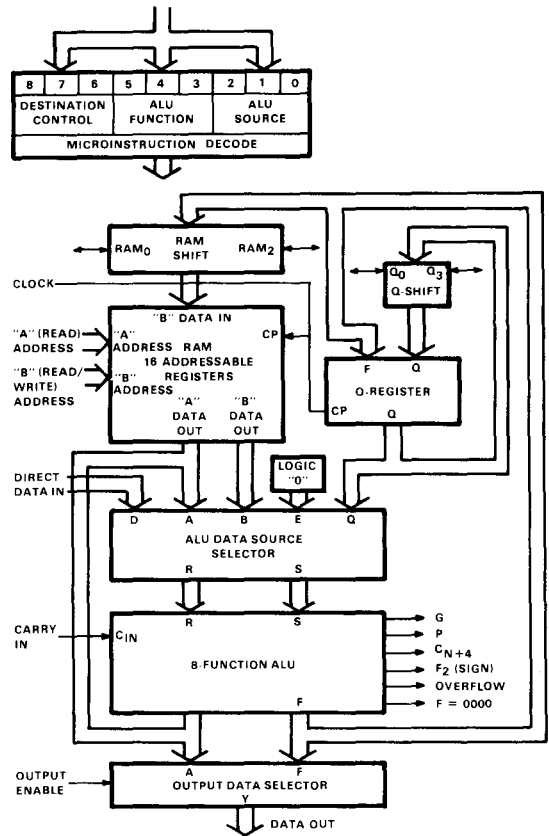
Figure 3. AMD2900 four-bit microprocessor slice block diagram (registers and data path).
