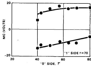
Figure 11. Tau margins.
