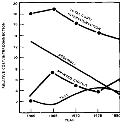
Figure 13. Relative cost per interconnection on DEC printed circuit board modules versus time.
