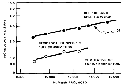
Figure 21. Technology progress functions for turbojet engines [Fusfeld, 1973].
