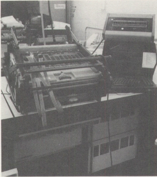
Figure 26. GenRad Corp. (GR) tester for modules.
