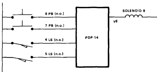
(c) Contact input (using normally open contacts) and solenoid output connections to PDP-14.
