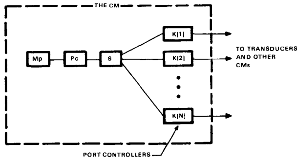
Figure 2. PMS diagram of Computer Module.
