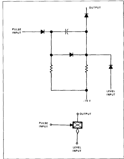
Figure 18. D-C-D gate.
