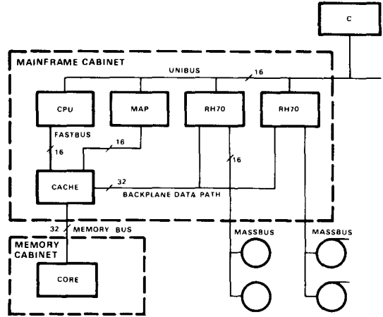
Figure 8. The PDP-11/70 configuration.
