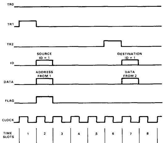
Figure 23. The timing of two SBI transfers which make up a read operation.
