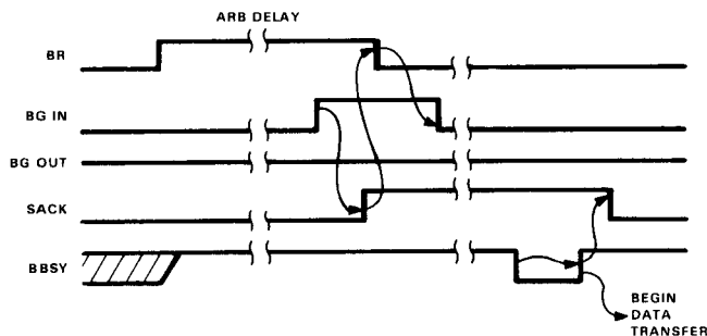
Figure 13. The timing of a Unibus arbitration sequence.
