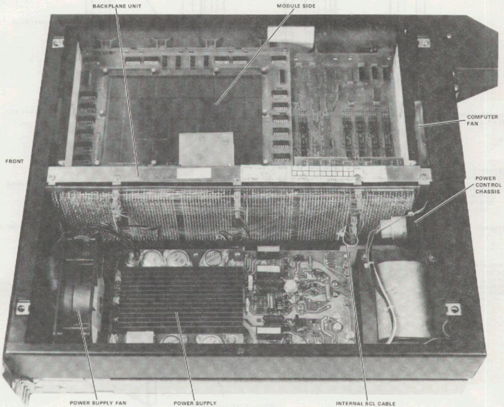
(b) Side view (with top cover removed).
