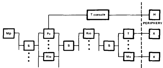
Figure 4. Conventional hierarchy computer structure.
