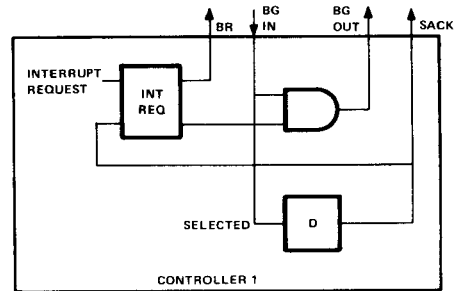
Figure 12. The arbitration logic of a controller attached to the Unibus.
