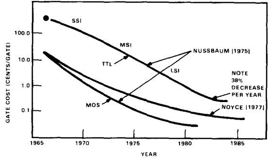
Figure 6. Price per gate versus time.
