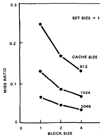
Figure 4. Effect of block size on miss ratio.
