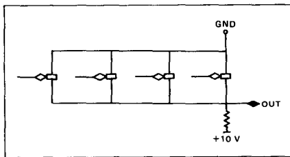
Figure 4. Parallel inverters.
