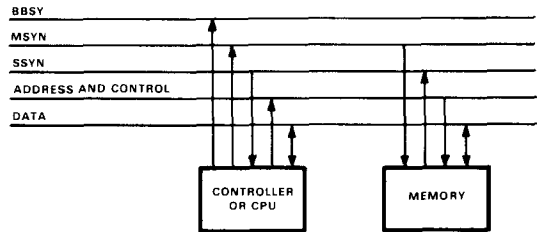
Figure 18. Unibus data transfer section.
