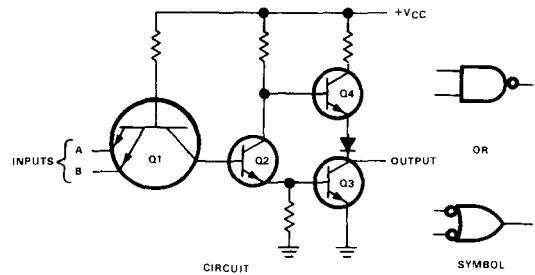
Figure 20. Basic TTL NAND gate circuit.
