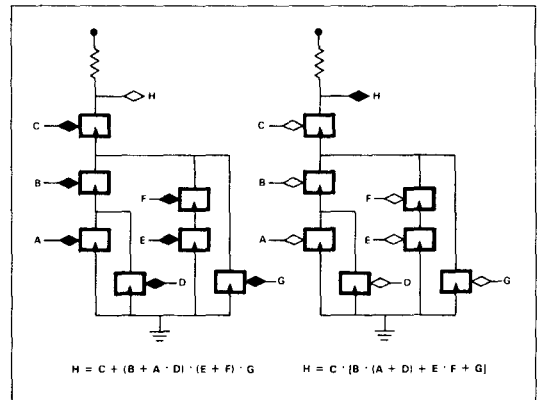
Figure 5. Sample circuits using series and parallel arrangements of inverters.
