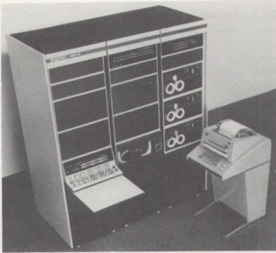
Figure 29. PDP-15/10.
