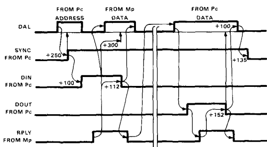
Figure 21. LSI-11 Bus Data-In-Out synchronization.
