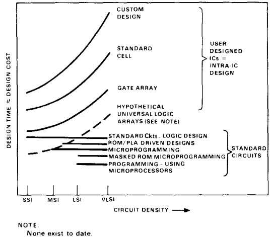
Figure 9. Current design cost (or time) versus circuit density using various design methods.
