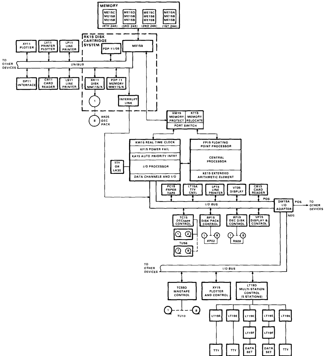
Figure 34. PDP-15/76 (XVM) system block diagram.
