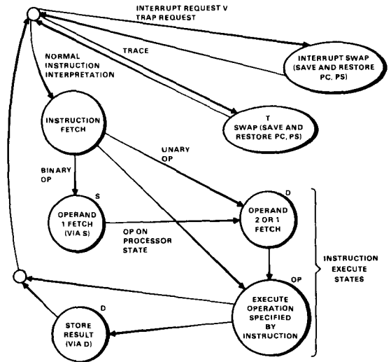
Figure 12. PDP-11 instruction interpretation process state diagram.
