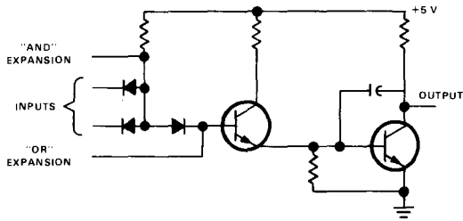
Figure 19. K-Series circuit.
