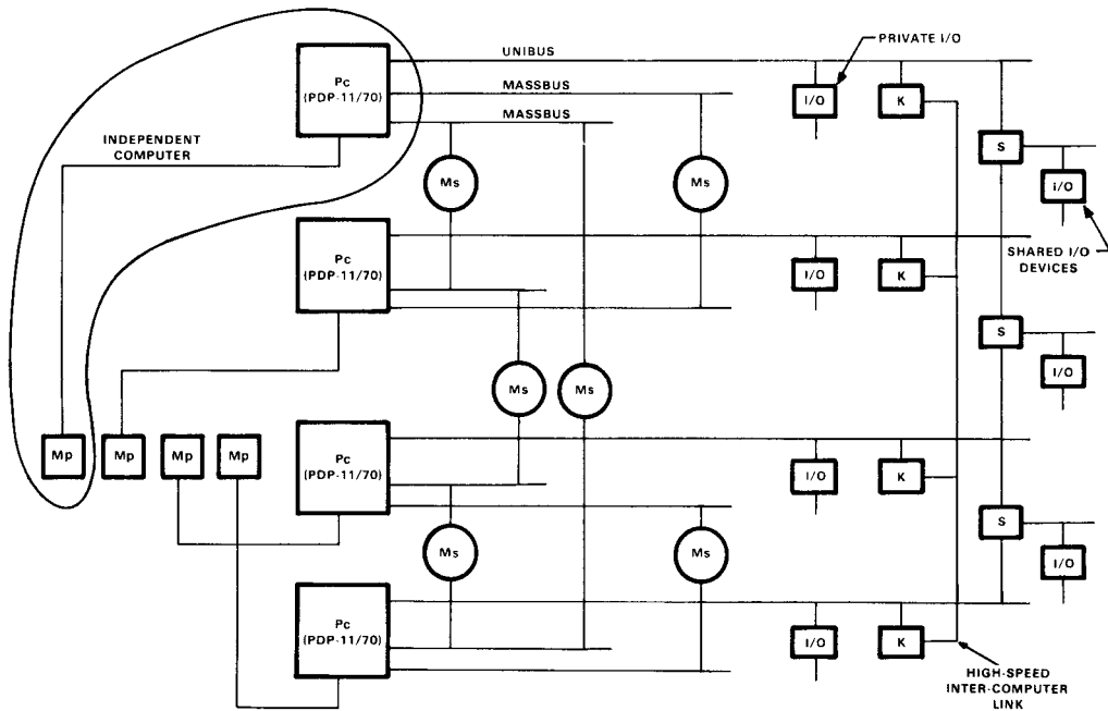
Figure 9. Four-processor multicomputer system based on PDP-11/70 processors.
