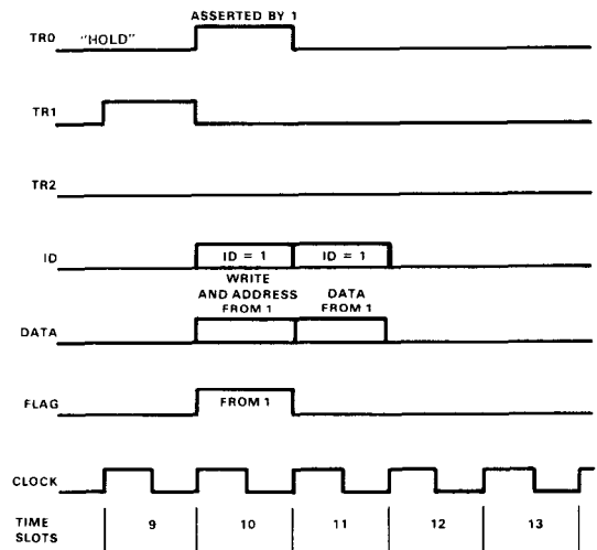
Figure 24. The timing of a memory write operation on the SBI.
