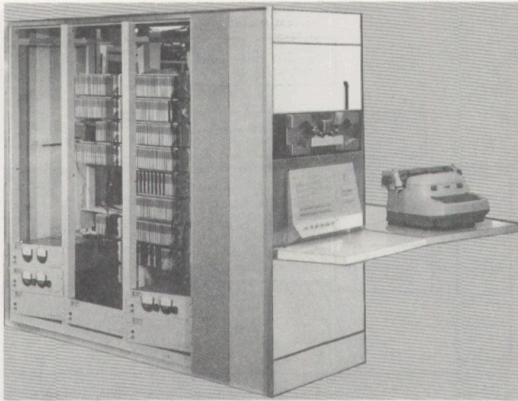
Figure 11. PDP-1/C production version (circa 1961).
