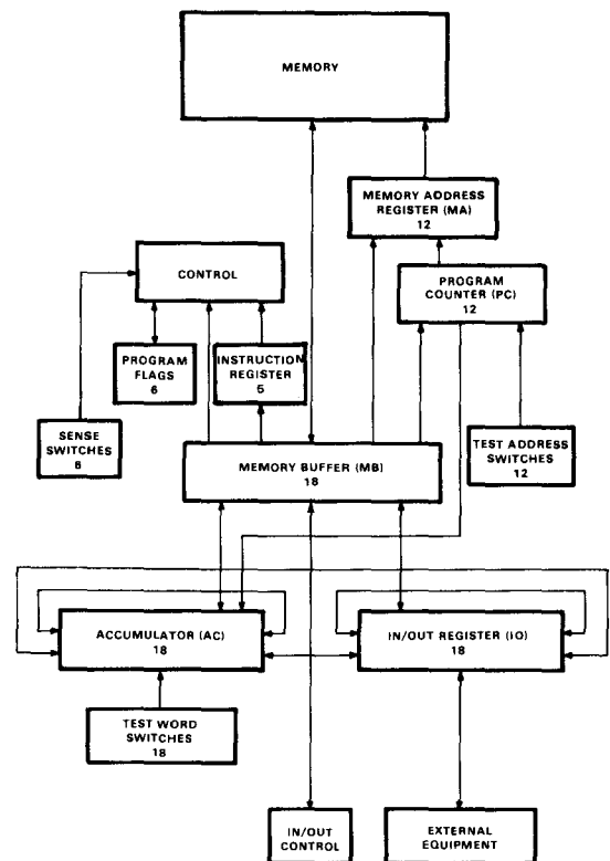
Figure 5. PDP-1 processor register transfer diagram.
