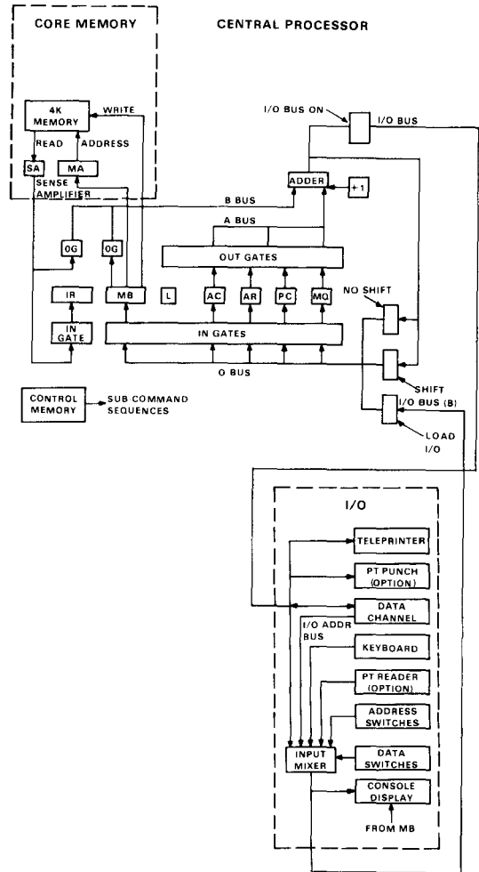
Figure 26. PDP-9 central processor register transfer diagram.
