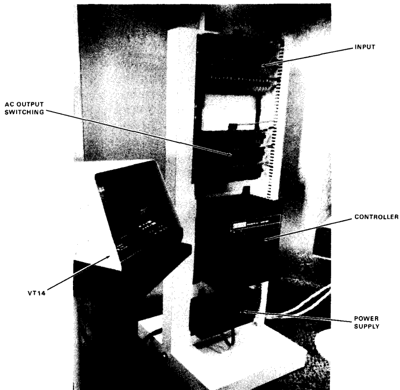
Figure 34. The PDP-14/30.
