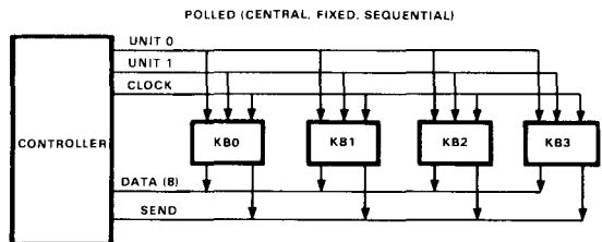
Figure 16. A hypothetical polled character-input bus.
