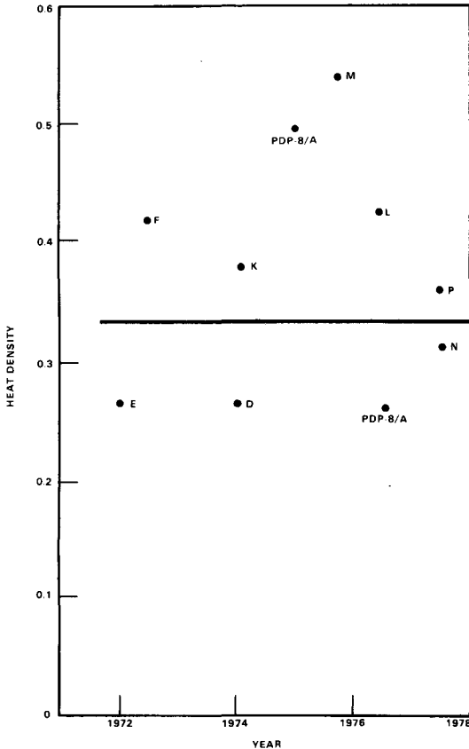
Figure 18. Heat density (kilowatts per ft 3 ) of various DEC computer boxes.
