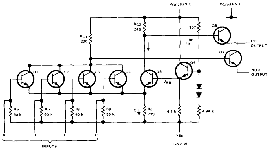
Figure 21. ECL circuit.
