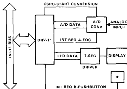
Figure 4. An interfacing example.
