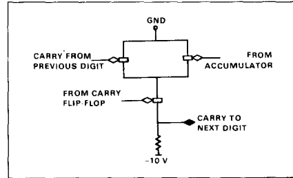
Figure 6. TX-2 carry circuits.
