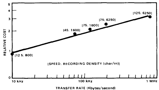
Figure 19. Relative cost versus transfer rate for various tape drives and controllers (1978).
