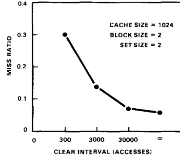
Figure 6. Effect of clear interval on miss ratio.
