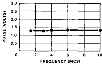
Figure 10. Trigger sensitivity.
