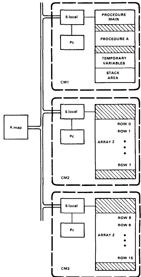
Figure 8. Physical layout of the program in memory.
