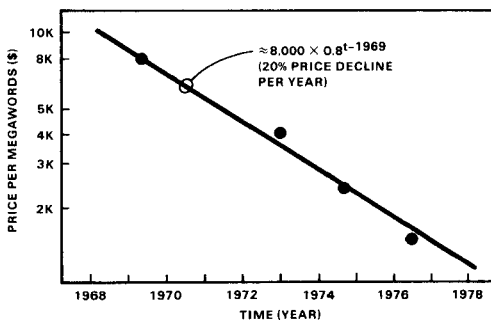
Figure 12. DECsystem-10 secondary memory price per Mwords versus time.
