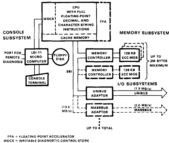
Figure 10. VAX-11/780 system.
