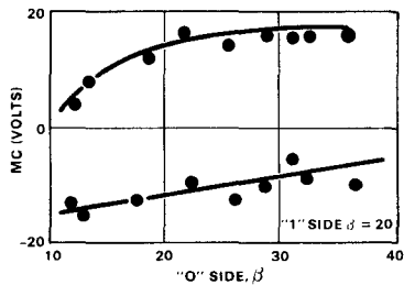
Figure 12. Beta margins.
