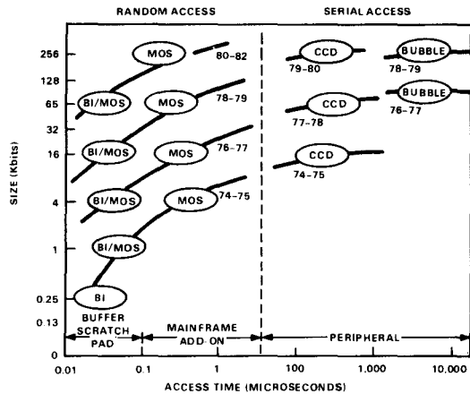
Figure 13. Memory size versus access time for various memories and yearly availability (courtesy of Dean Toombs, Texas Instruments, Inc.).
