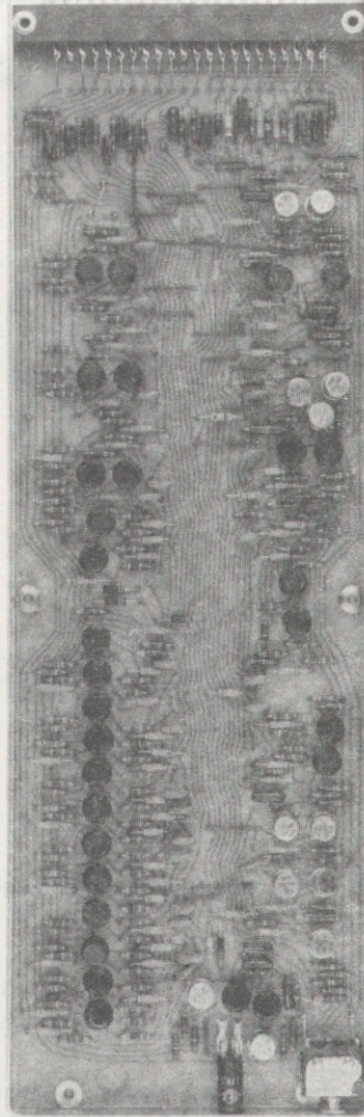
Figure 8. 4707 transmitter line unit of the late second generation.
