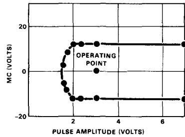
Figure 16. Pulse margins.
