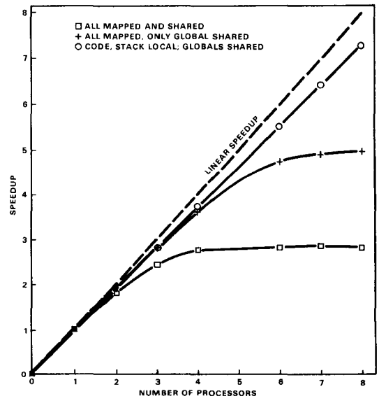
Figure 20. PDE speedup.
