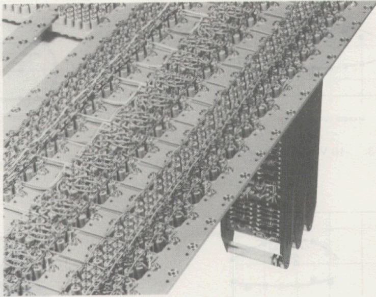
Figure 18. TX-2 back panel.
