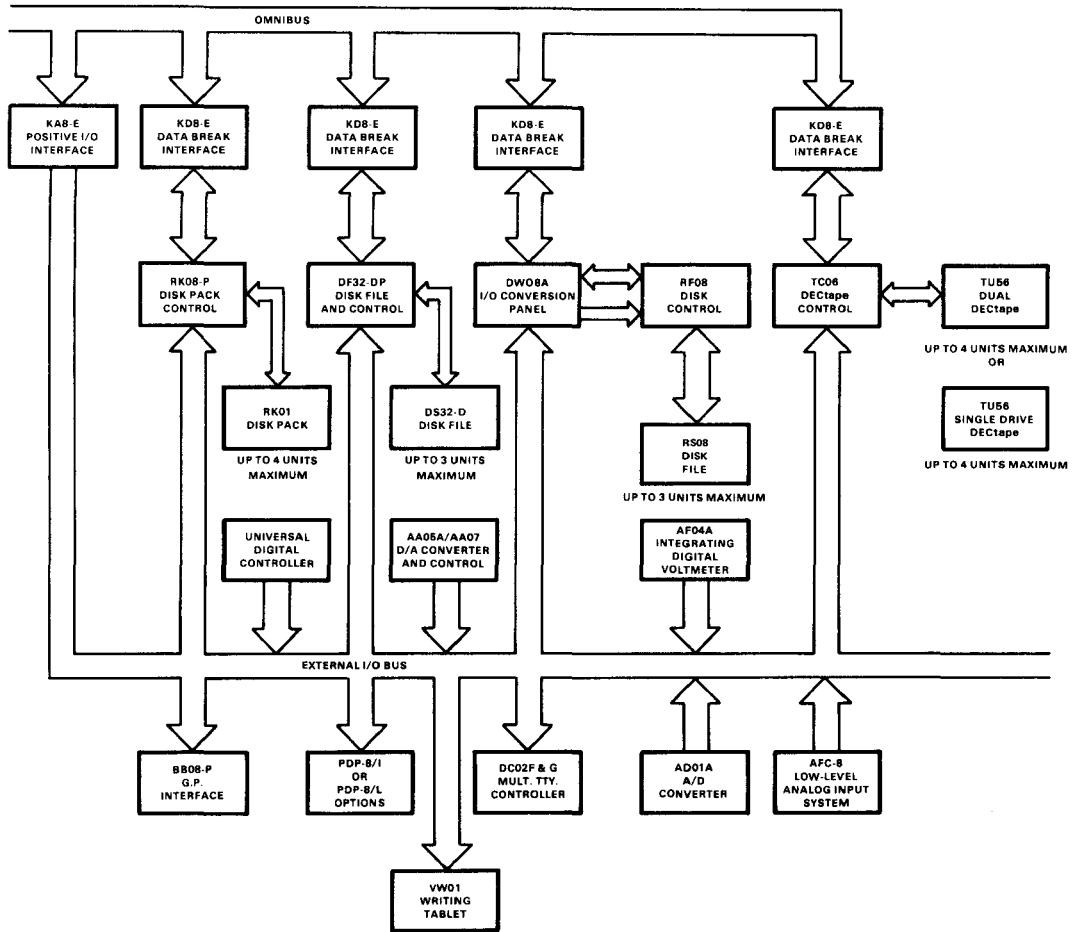
Figure 12. PDP-8/E system block diagram (part 2 of 2).
