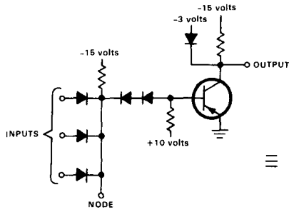
(a) Multiple input inverter circuit.
