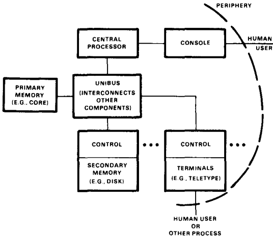
(a) Conventional block diagram.
