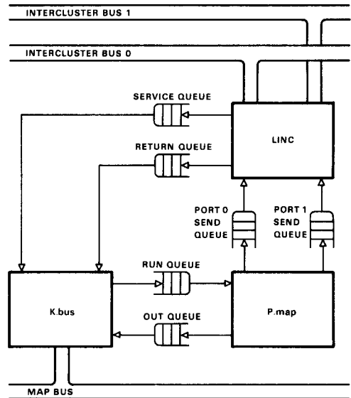
Figure 14. The components of a K.map.
