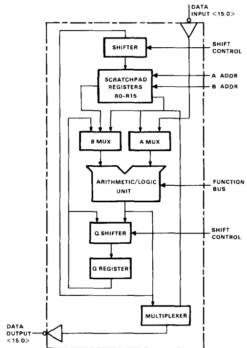
Figure 5. The AM2901 – a 4-bit bipolar microprocessor slice.
