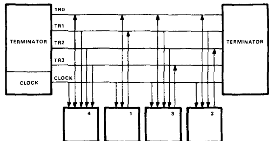
Figure 14. A simplified diagram of SBI arbitration signals.
