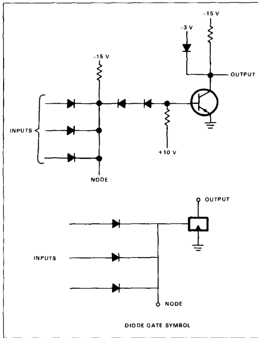
Figure 17. Diode gate.
