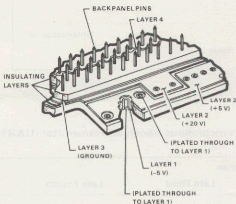
Figure 5. Cross-section of a printed circuit backplane.
