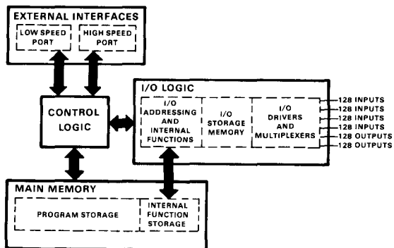
Figure 35. Block diagram of PDP-14/30.
