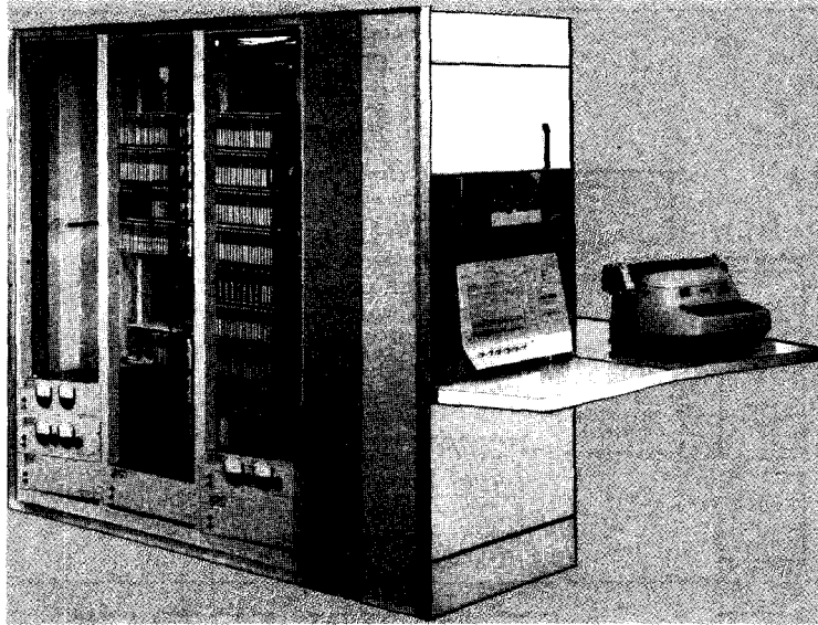
Figure 11. PDP-1/C production version (circa 1961).
