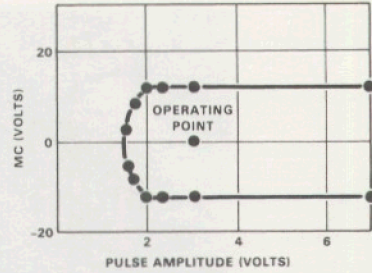
Figure 16. Pulse margins.
