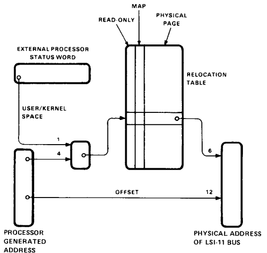
Figure 11. Virtual-to-physical address translation for a local memory reference.
