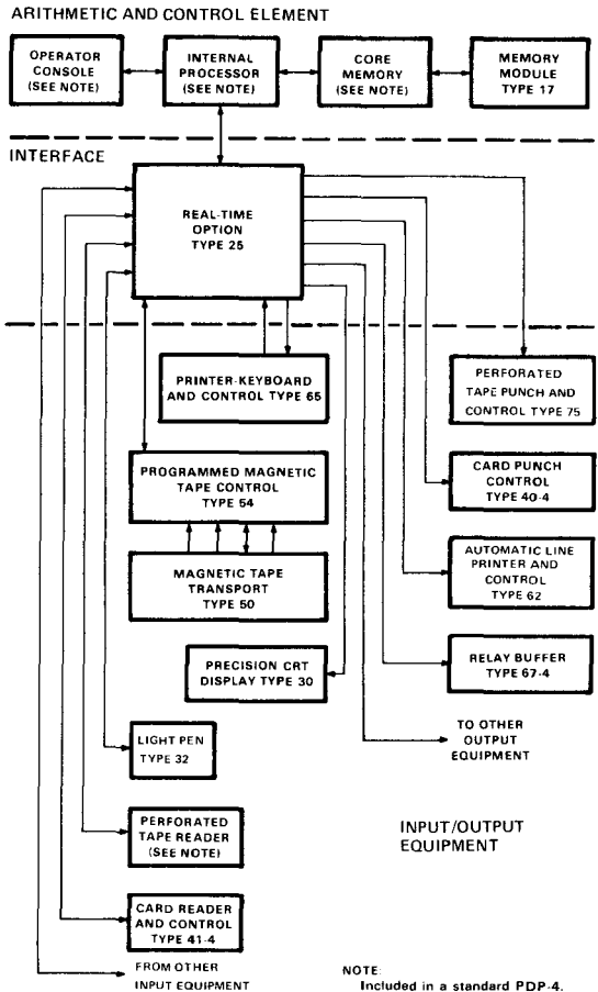
Figure 16. PDP-4 block diagram.
