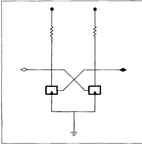
Figure 9. Primitive flip-flop.
