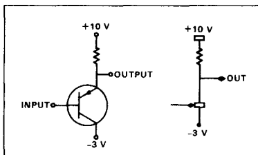
Figure 1. Emitter follower.
