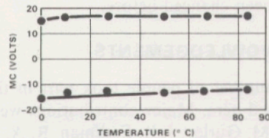
Figure 15. Temperature margins.
