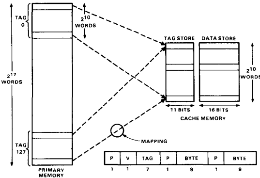
Figure 5. Direct-mapped cache. Mapping occurs from 128 Kwords of primary memory to 1024-word cache. High-order seven bits of an 18-bit address are stored in tag store to ensure uniqueness in mapping. Tag store also holds a valid bit and parity bits. Cache word format (27 bits in total) is as shown in the bit map.
