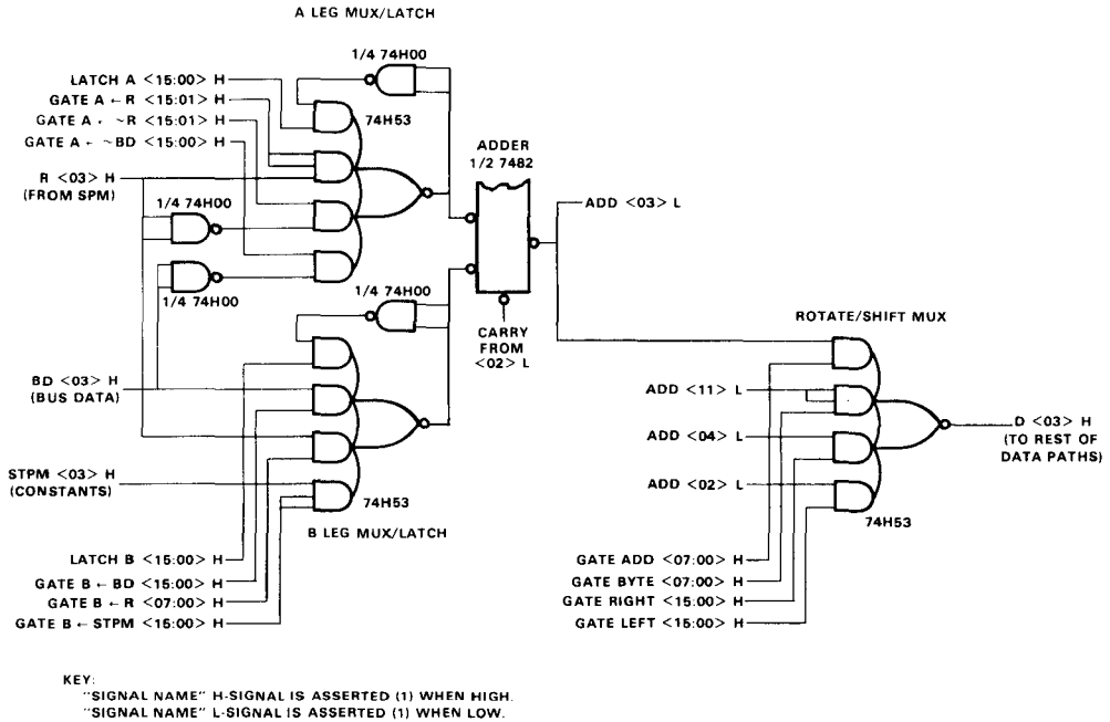
Figure 5. Detail of central part of PDP-11/20 data paths. One-bit (03) slice (adapted from KC11 Processor Manual ).
