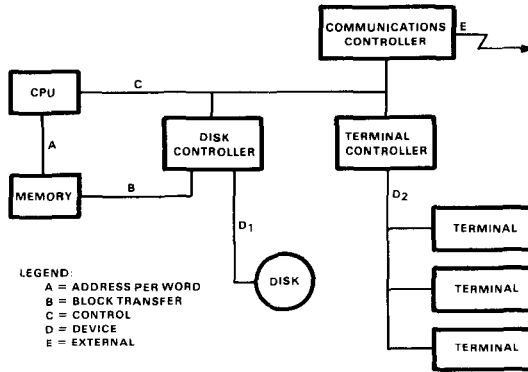
Figure 4. A five-function model of computer buses.
