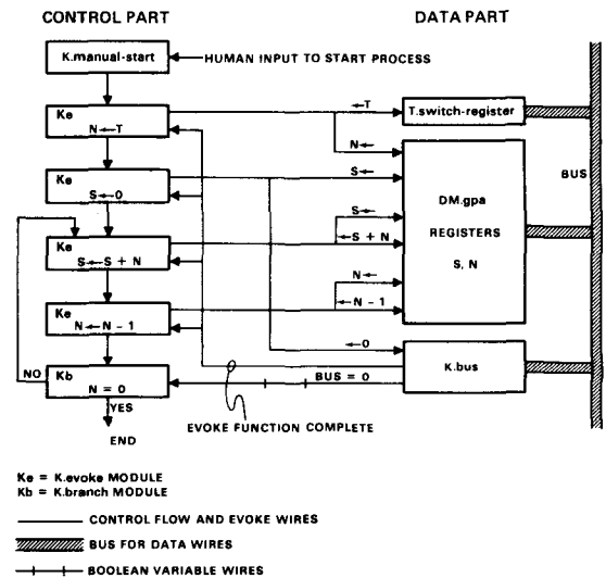
Figure 3. RTM digital system to take a value from a switch register input and to sum the integers to the input value.
