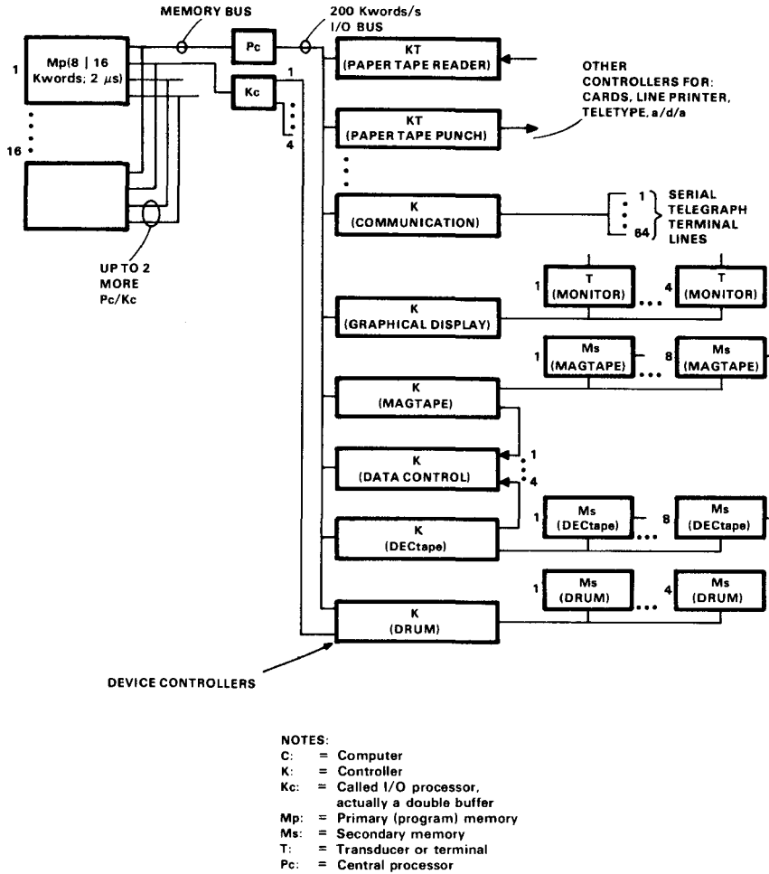
Figure 3. PMS diagram for PDP-6 system.
