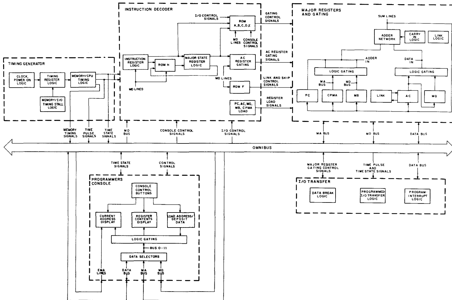
Figure 14. PDP-8/A processor and register transfer diagram.
