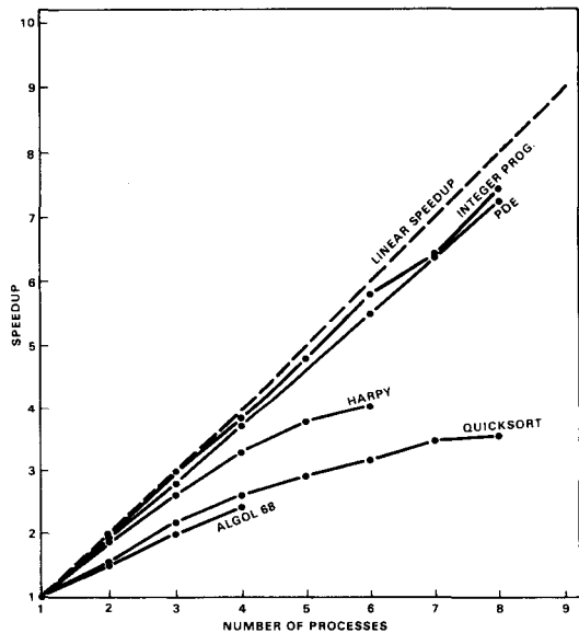
Figure 18. Average speedup of five algorithms of Cm*
