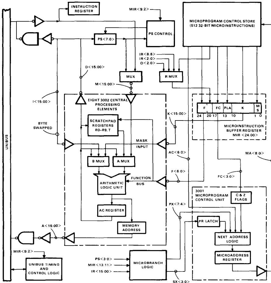
Figure 1. Register transfer level diagram.
