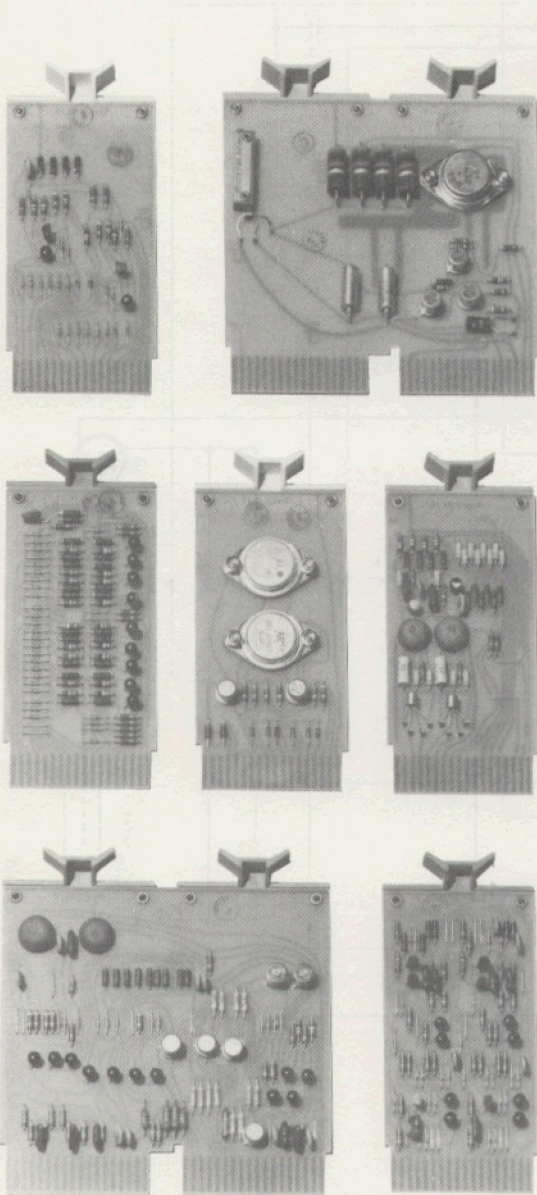
Figure 16. Single and double Flip Chip modules used in PDP-7 and PDP-8.
