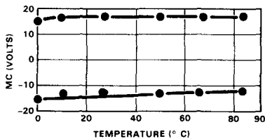
Figure 15. Temperature margins.
