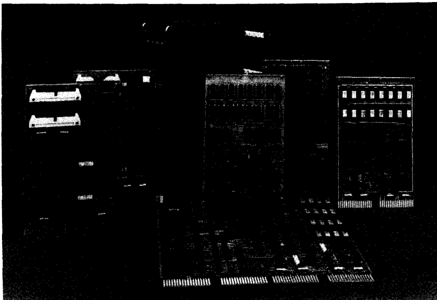
Figure 5. The LSI-11 series contains the LSI-11 CPU (center), together with parallel and serial interfaces, and RAM and ROM memory modules. These modules may be housed in a backplane assembly, connected by the LSI-11 bus.
