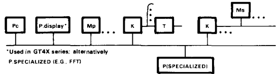
(b) Pc with P.display using a single Unibus.
