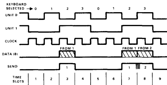
Figure 17. Timing diagram of a polled character-input bus.
