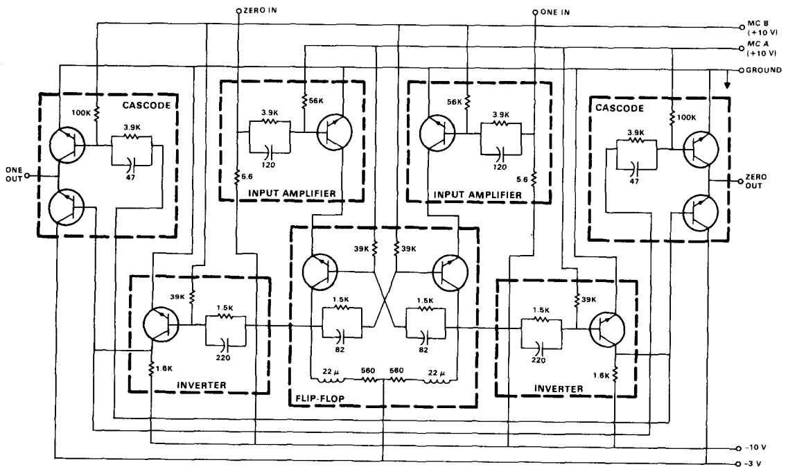
Figure 8. TX-2 flip-flop.
