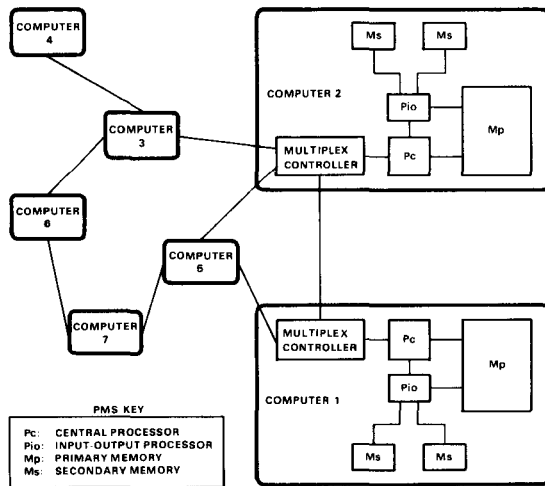
Figure 2. A network of computers.
