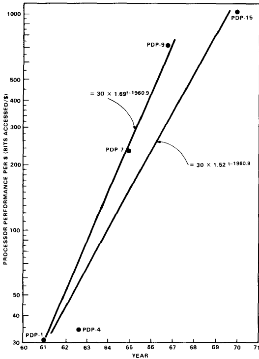
Figure 38. Processor performance per $ versus time of 18-bit machines.
