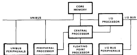
Figure 33. PDP-15/76 simple system block diagram.
