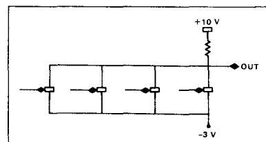
Figure 2. Parallel emitter follower.
