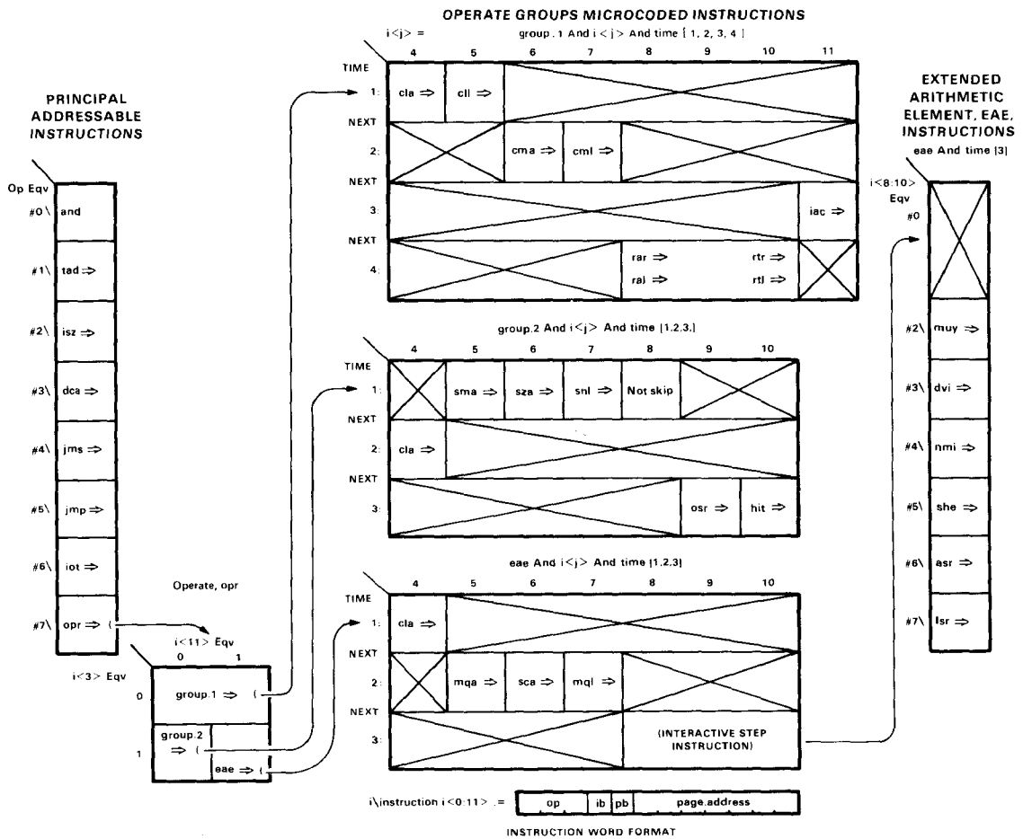
Figure 5. PDP-8 instruction decoding diagram.
