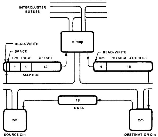
Figure 13. The mechanism for external references.
