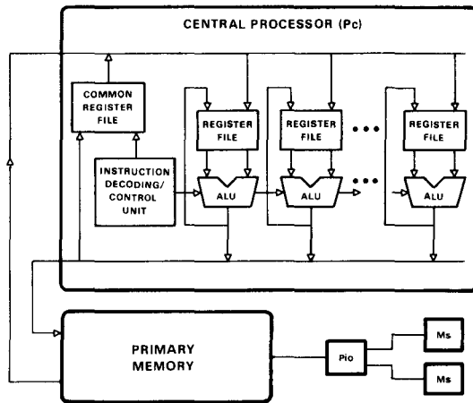
Figure 4. Multi-ALU processor.
