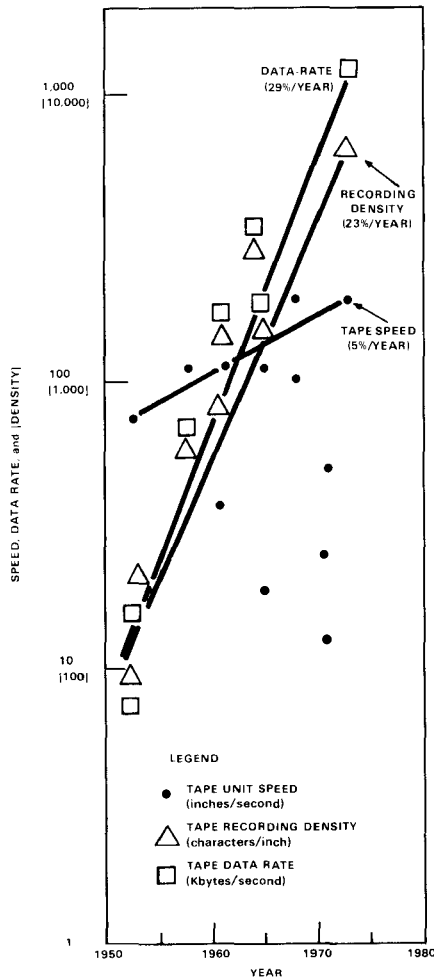
Figure 18. Characteristics of various IBM magnetic tape units versus time.
