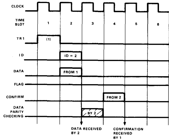
Figure 31. Timing of SBI data transfer acknowledgements, including parity check.
