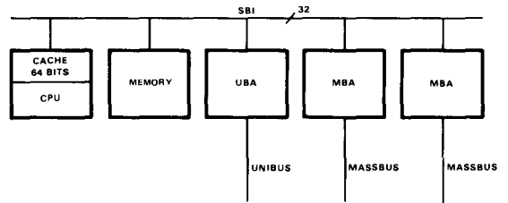
Figure 9. The VAX-11/780 organization, based on the SBI.
