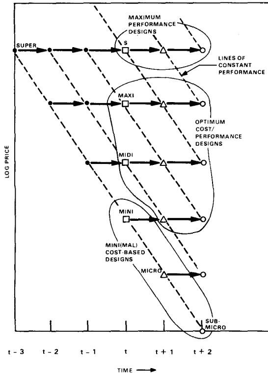
Figure 11. Price versus time for each machine class.
