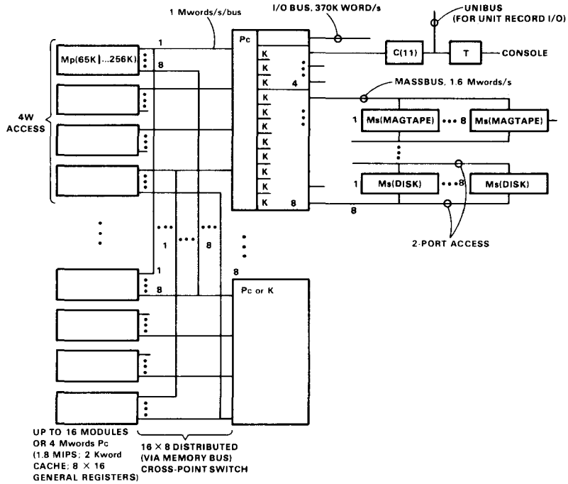
Figure 6. PMS diagram for KL10 processor-based system.
