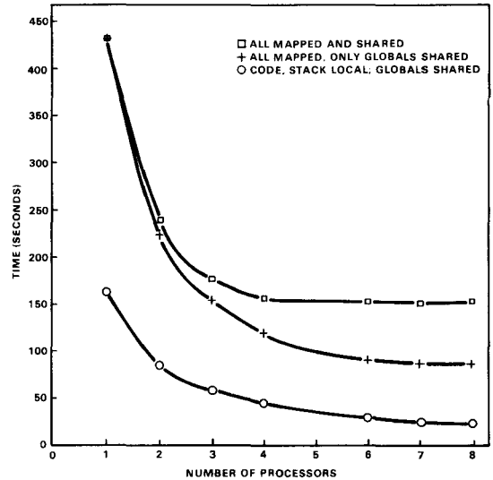
Figure 19. PDE execution time.
