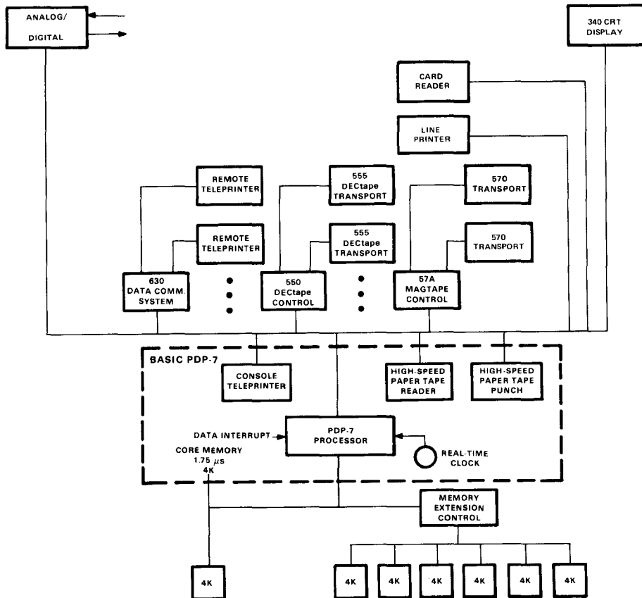
Figure 22. PDP-7 system block diagram.
