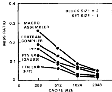
Figure 2. Effect of cache size on miss ratio.
