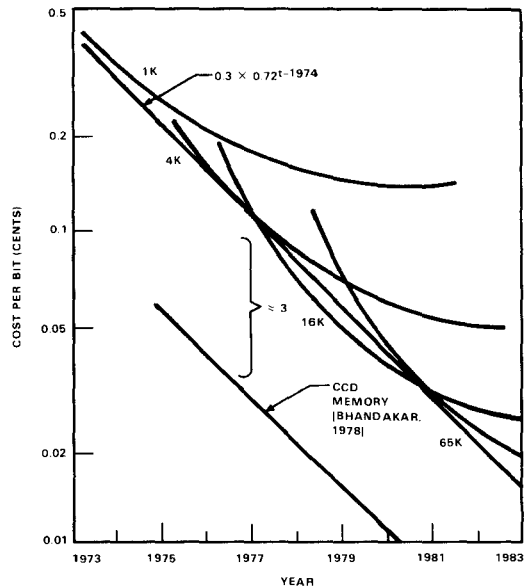
Figure 7. Cost per bit of integrated circuit memory versus time. Cost per bit of computer memory has declined and should continue to decline as is shown here for successive generations of random-access memory circuits capable of handling from 1,024 (1 K) to 65,536 (65 K) bits of memory. Increasing complexity of successive circuits is primarily responsible for cost reduction, but less complex circuits also continue to decline in cost (adapted from [Noyce, 1977: 69]; courtesy of Scientific American ).
