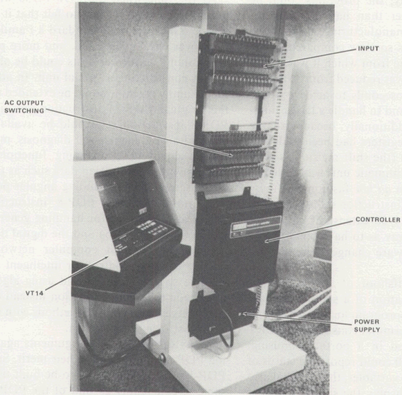
Figure 34. The PDP-14/30.
