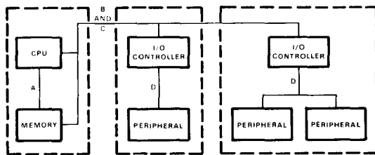
(b) Single types B and C pathways, extending out of the "mainframe" package; short type D paths.
