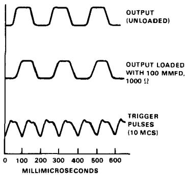
Figure 9. Flip-flop waveforms.
