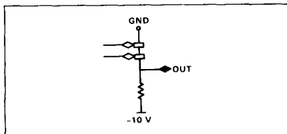
Figure 5. Series inverters.
