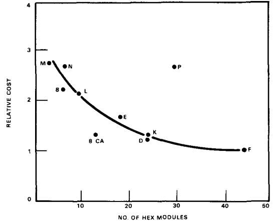
Figure 21. Relative cost of box materials versus number of hex size modules for various DEC minicomputer boxes.
