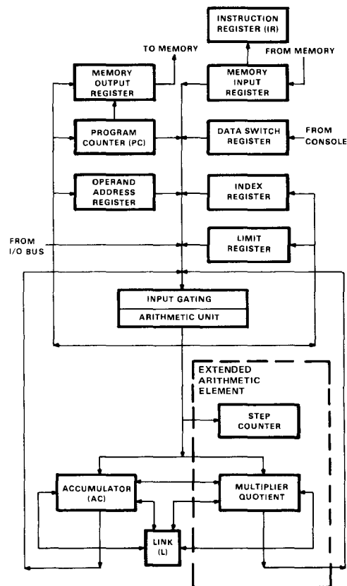
Figure 31. PDP-15 processor register transfer diagram.
