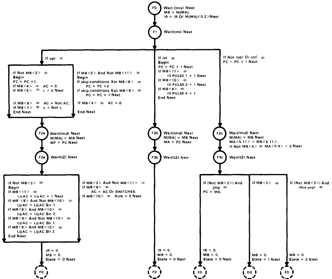
Figure 7. PDP-8 Pc state diagram (part 1 of 2).
