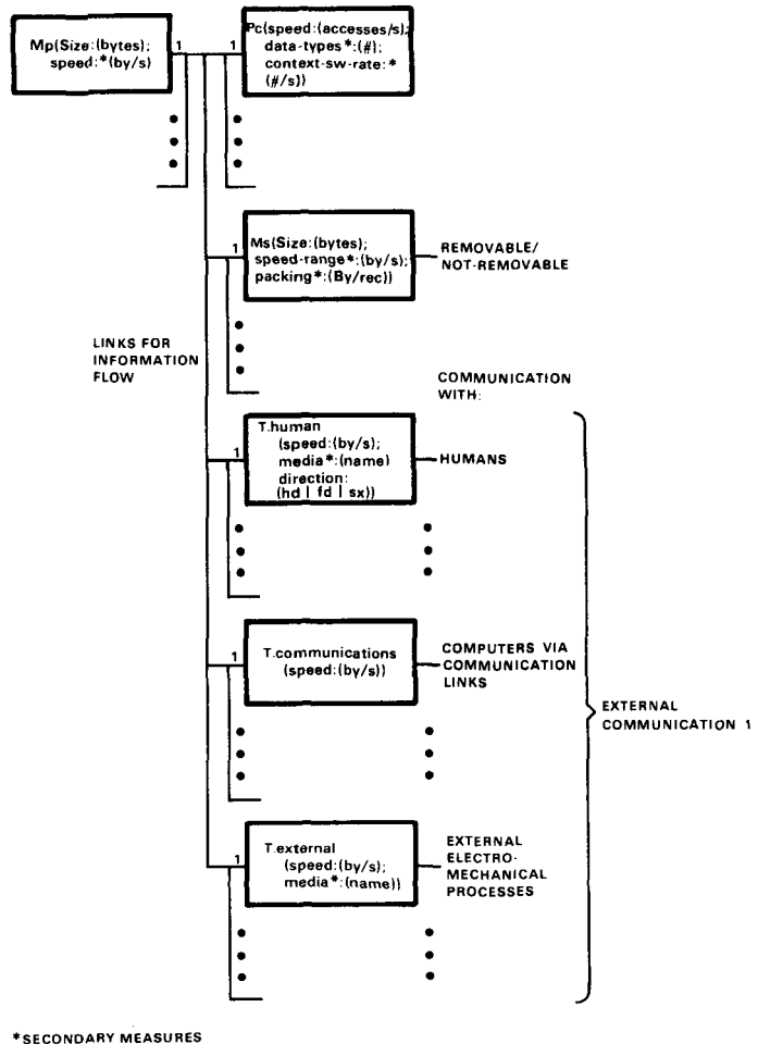
Figure 1. Basic PMS computer structure model with six relevant performance/structure dimensions.
