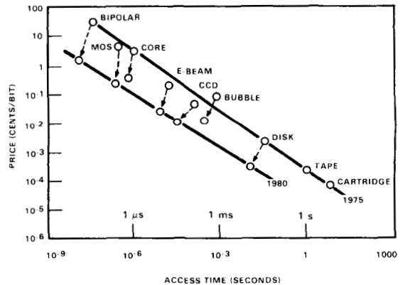
Figure 17. Memory trends, 1975–1980 (courtesy of Memorex Corporation, 1978).
