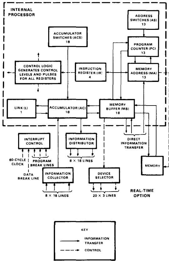
Figure 15. PDP-4 processor/real-time option register transfer diagram.
