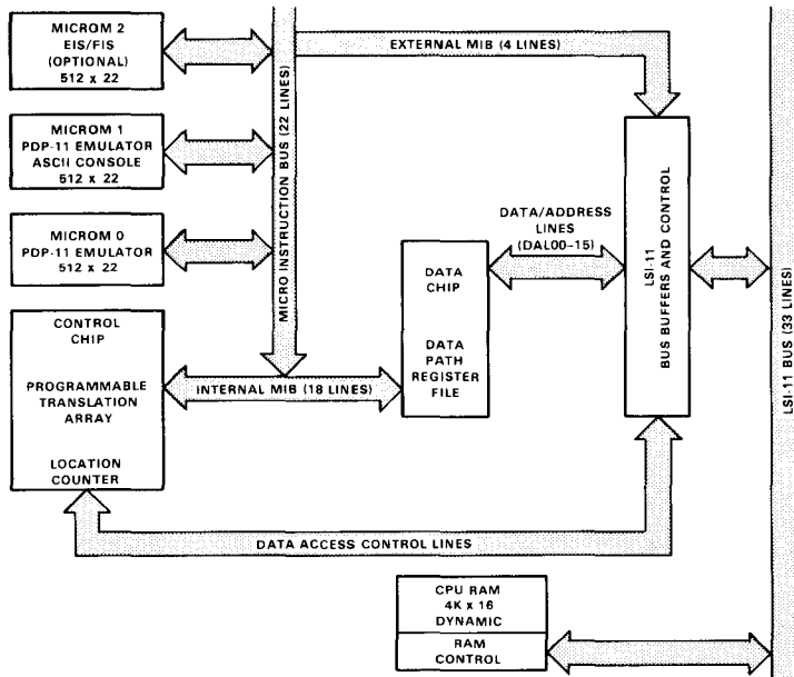
Figure 2. Organization of the LSI-11 CPU.
