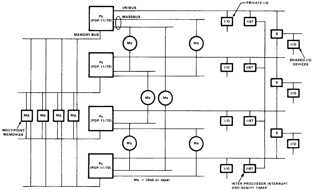
Figure 8. Four-processor multiprocessor based on PDP-11/70 processors.
